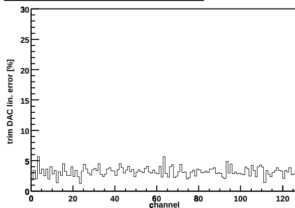
Chip Z36459A-W04-X15-Y13 trim DAC lin. error
