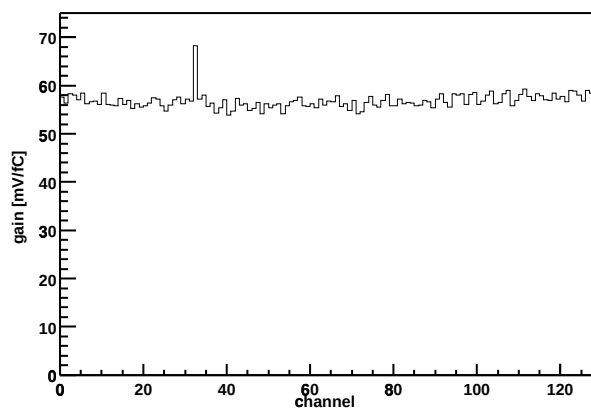
Chip Z36459A-W04-X15-Y13 Gain vs. channel
