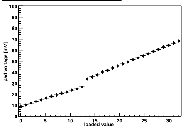
Chip Z36459A-W04-X15-Y13 shaper DAC
