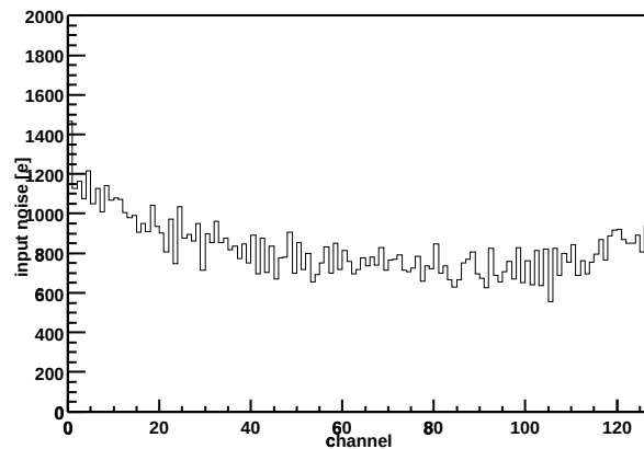
Chip Z36459A-W04-X15-Y13 Input noise vs. channel
