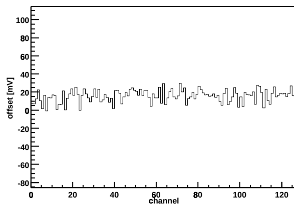
Chip Z36459A-W04-X15-Y13 Offset vs. channel
