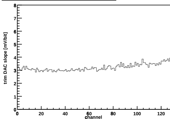
Chip Z36459A-W04-X15-Y13 Trim DAC slope vs. channel
