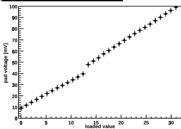
Chip Z36459A-W04-X15-Y13 preamp DAC
