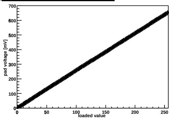
Chip Z36459A-W04-X15-Y13 threshold DAC
