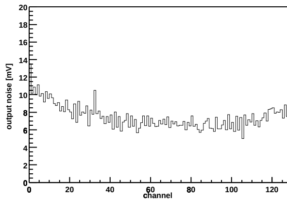
Chip Z36459A-W04-X15-Y13 Output noise vs. channel
