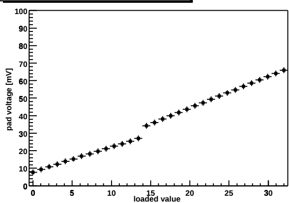
Chip Z36459A-W04-X16-Y09 shaper DAC
