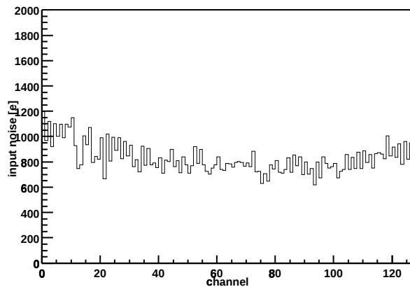
Chip Z36459A-W04-X16-Y09 Input noise vs. channel
