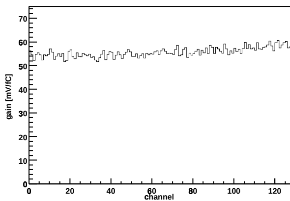
Chip Z36459A-W04-X16-Y09 Gain vs. channel
