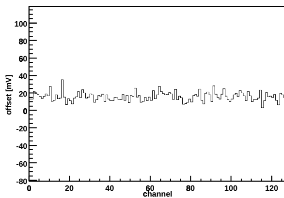
Chip Z36459A-W04-X16-Y09 Offset vs. channel
