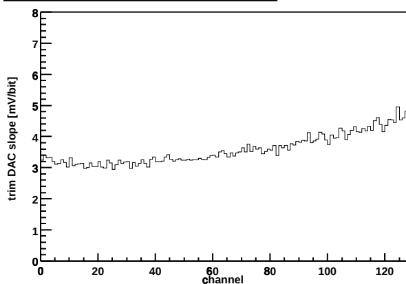
Chip Z36459A-W04-X16-Y09 Trim DAC slope vs. channel
