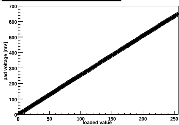
Chip Z36459A-W04-X16-Y09 threshold DAC
