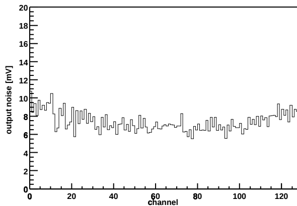
Chip Z36459A-W04-X16-Y09 Output noise vs. channel
