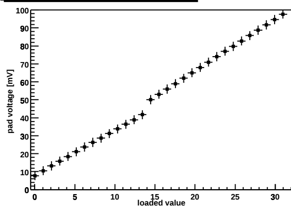
Chip Z36459A-W04-X16-Y09 preamp DAC
