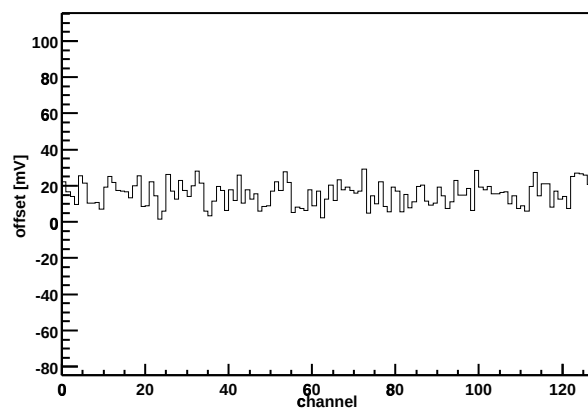
Chip Z36459A-W06-X01-Y08 Offset vs. channel
