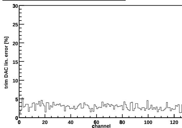
Chip Z36459A-W06-X01-Y08 trim DAC lin. error
