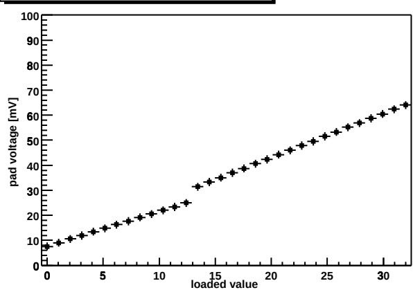
Chip Z36459A-W06-X01-Y08 shaper DAC
