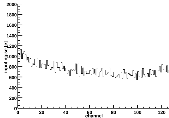
Chip Z36459A-W06-X01-Y08 Input noise vs. channel
