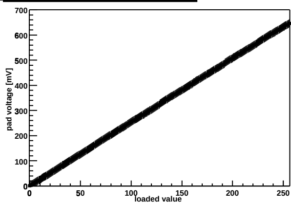
Chip Z36459A-W06-X01-Y08 threshold DAC
