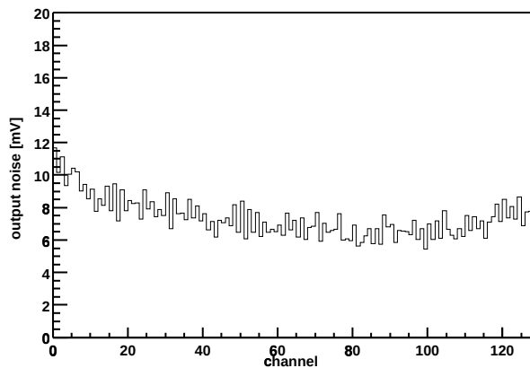
Chip Z36459A-W06-X01-Y08 Output noise vs. channel
