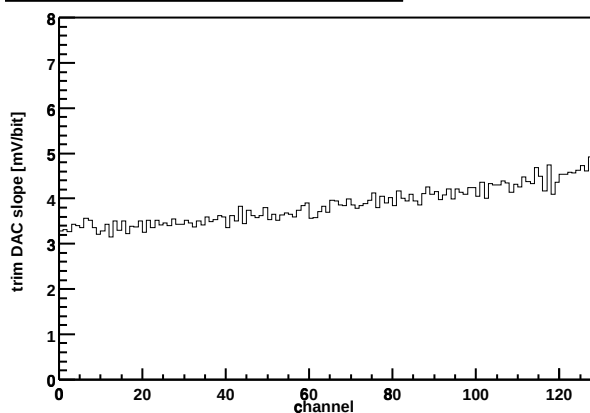
Chip Z36459A-W06-X01-Y08 Trim DAC slope vs. channel
