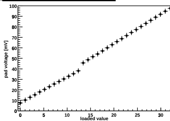
Chip Z36459A-W06-X01-Y08 preamp DAC
