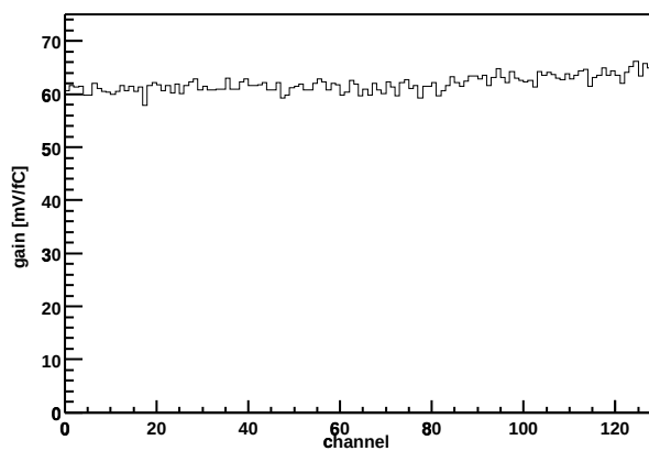
Chip Z36459A-W06-X01-Y08 Gain vs. channel
