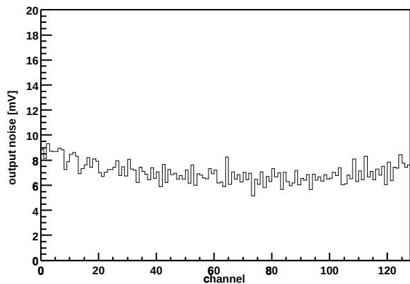
Chip Z36459A-W06-X02-Y15 Output noise vs. channel
