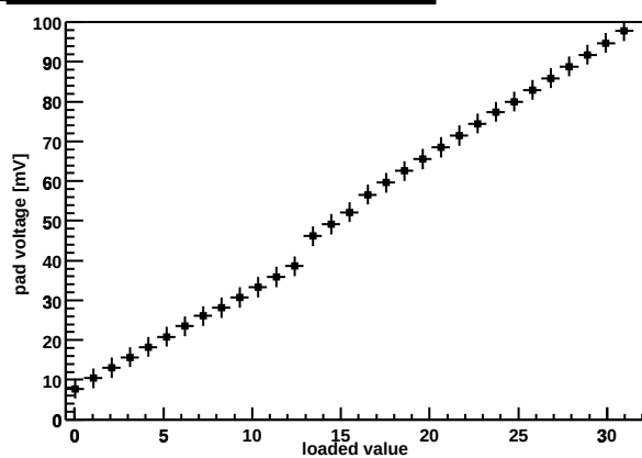
Chip Z36459A-W06-X02-Y15 preamp DAC
