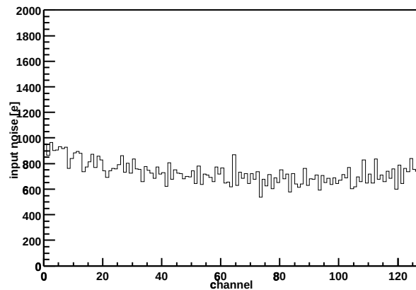
Chip Z36459A-W06-X02-Y15 Input noise vs. channel
