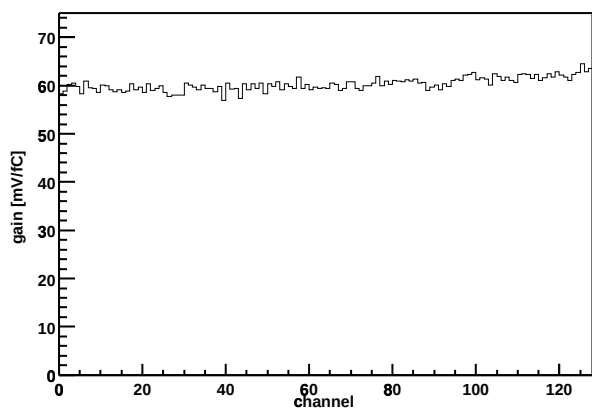
Chip Z36459A-W06-X02-Y15 Gain vs. channel
