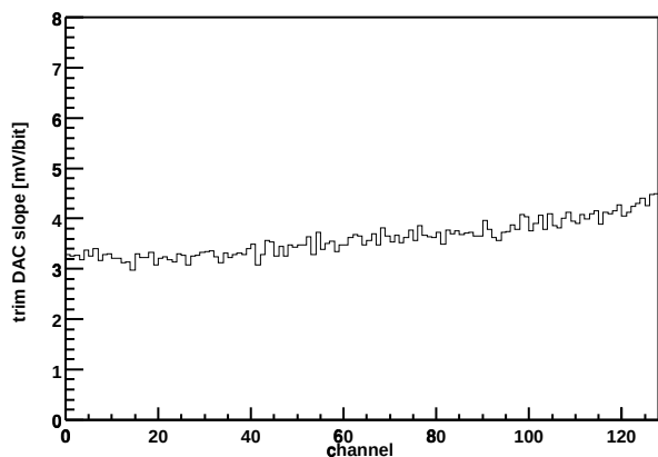
Chip Z36459A-W06-X02-Y15 Trim DAC slope vs. channel
