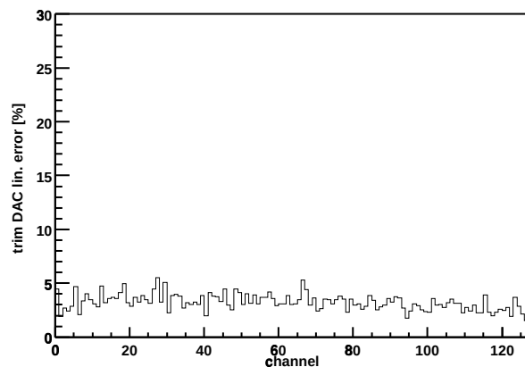
Chip Z36459A-W06-X02-Y15 trim DAC lin. error
