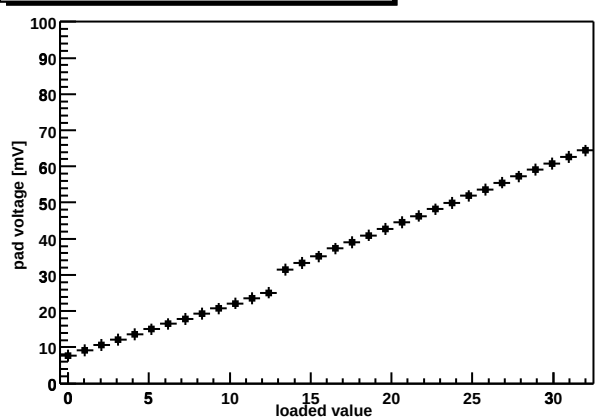
Chip Z36459A-W06-X02-Y15 shaper DAC
