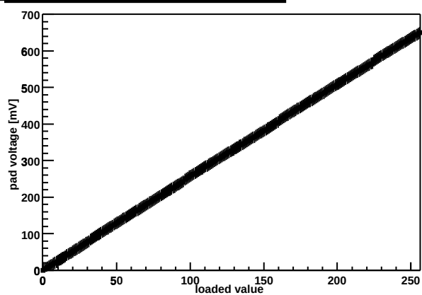
Chip Z36459A-W06-X02-Y15 threshold DAC
