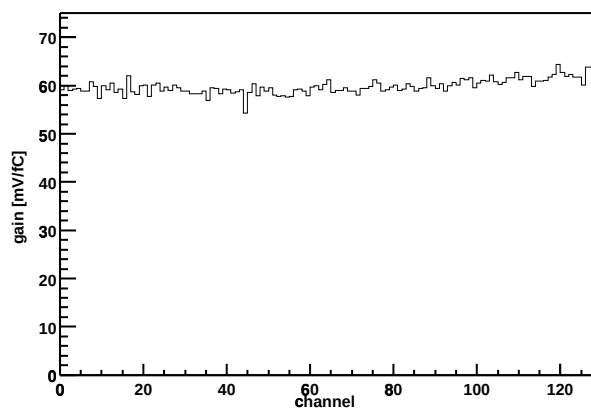
Chip Z36459A-W06-X03-Y12 Gain vs. channel
