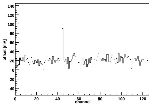
Chip Z36459A-W06-X03-Y12 Offset vs. channel
