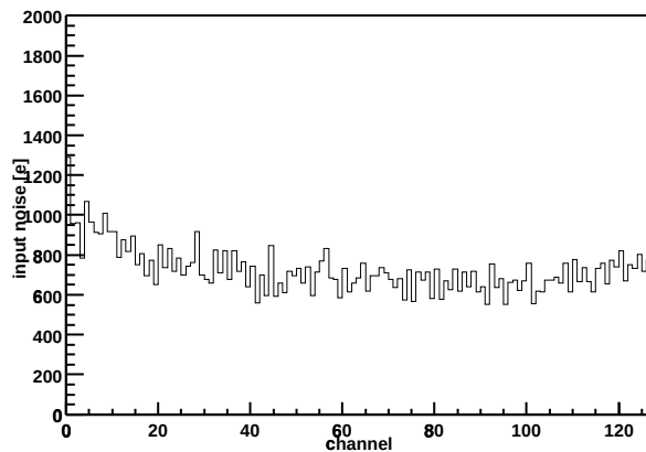
Chip Z36459A-W06-X03-Y12 Input noise vs. channel
