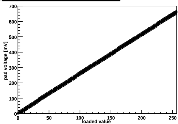
Chip Z36459A-W06-X03-Y12 threshold DAC
