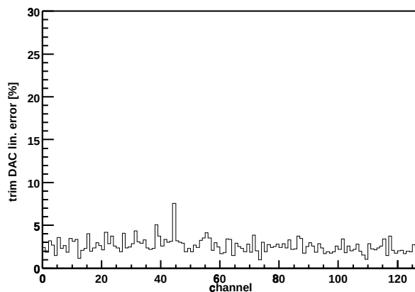
Chip Z36459A-W06-X03-Y12 trim DAC lin. error
