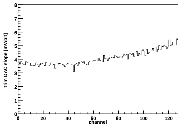
Chip Z36459A-W06-X03-Y12 Trim DAC slope vs. channel
