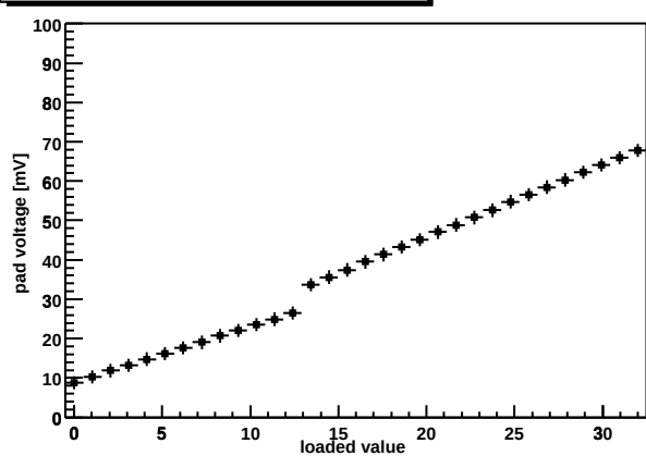
Chip Z36459A-W06-X03-Y12 shaper DAC
