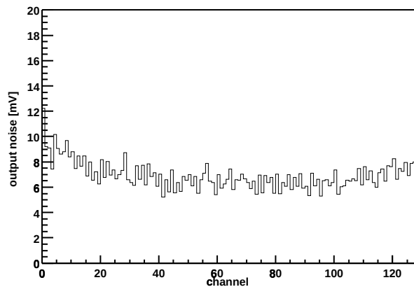
Chip Z36459A-W06-X03-Y12 Output noise vs. channel
