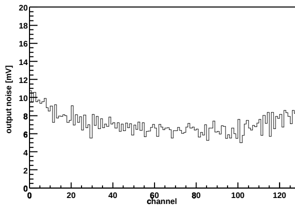
Chip Z36459A-W06-X03-Y14 Output noise vs. channel
