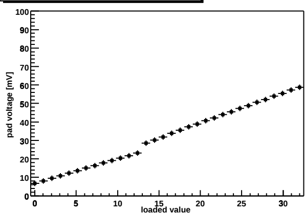
Chip Z36459A-W06-X03-Y14 shaper DAC
