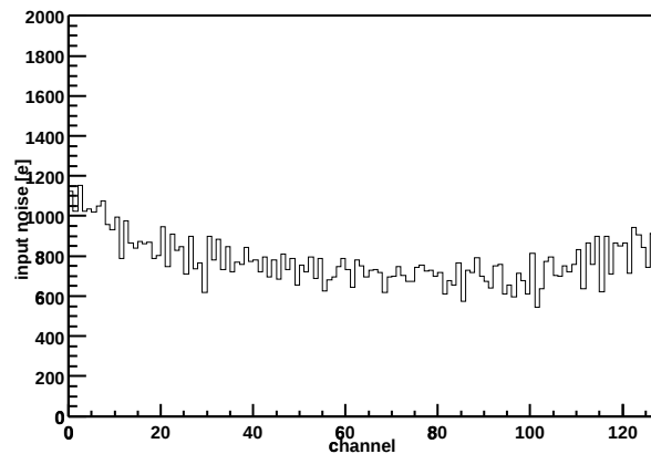
Chip Z36459A-W06-X03-Y14 Input noise vs. channel
