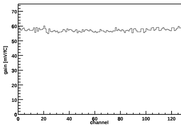
Chip Z36459A-W06-X03-Y14 Gain vs. channel
