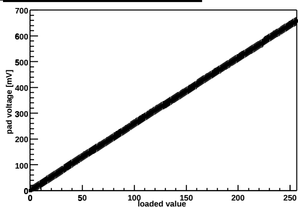
Chip Z36459A-W06-X03-Y14 threshold DAC
