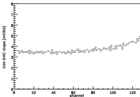
Chip Z36459A-W06-X03-Y14 Trim DAC slope vs. channel
