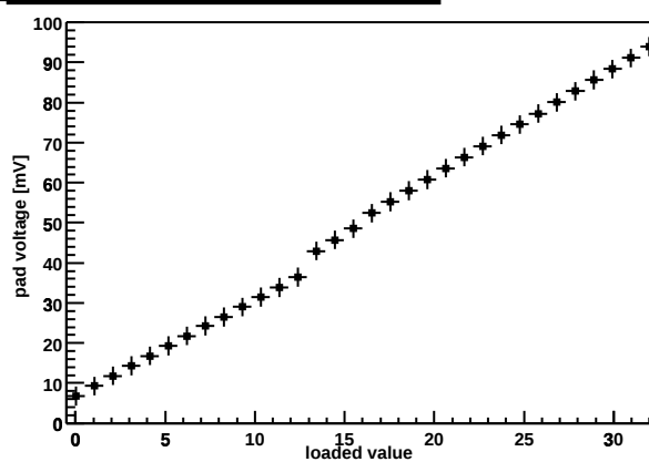
Chip Z36459A-W06-X03-Y14 preamp DAC
