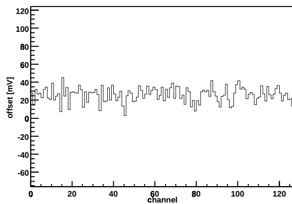
Chip Z36459A-W06-X03-Y14 Offset vs. channel
