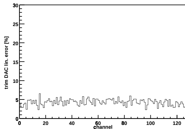
Chip Z36459A-W06-X03-Y14 trim DAC lin. error
