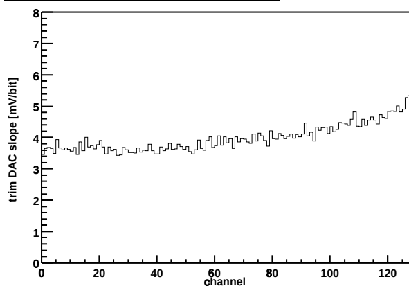
Chip Z36459A-W06-X04-Y07 Trim DAC slope vs. channel
