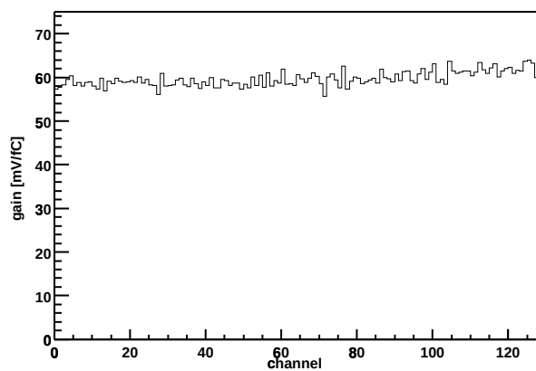
Chip Z36459A-W06-X04-Y07 Gain vs. channel
