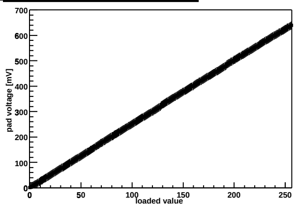
Chip Z36459A-W06-X04-Y07 threshold DAC
