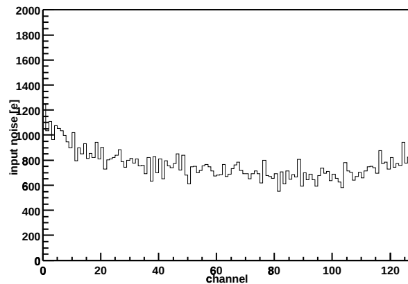
Chip Z36459A-W06-X04-Y07 Input noise vs. channel
