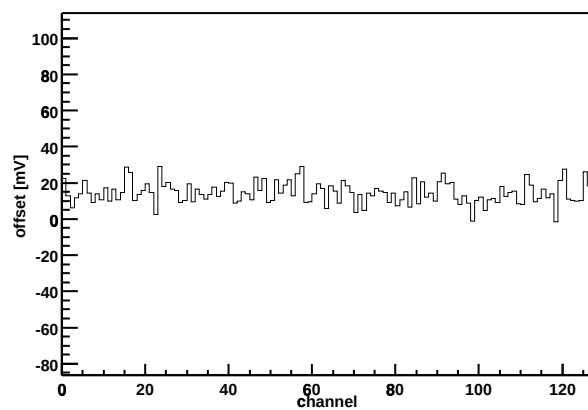
Chip Z36459A-W06-X04-Y07 Offset vs. channel
