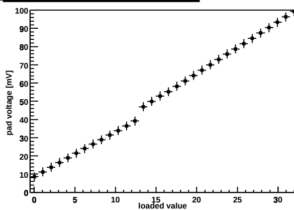
Chip Z36459A-W06-X04-Y07 preamp DAC
