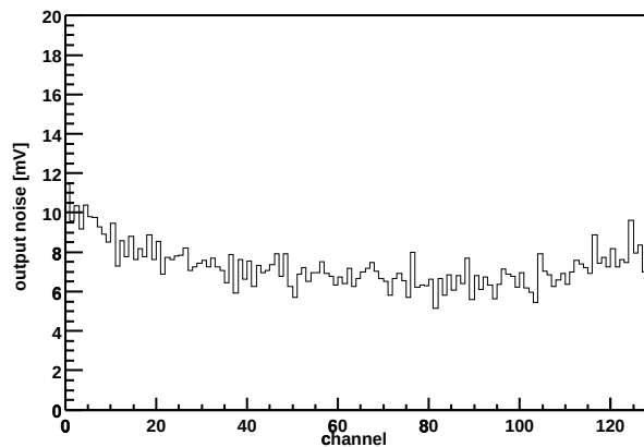
Chip Z36459A-W06-X04-Y07 Output noise vs. channel
