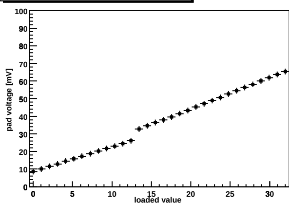
Chip Z36459A-W06-X04-Y07 shaper DAC
