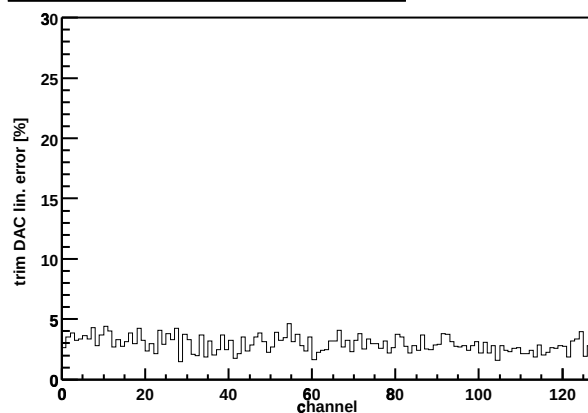
Chip Z36459A-W06-X04-Y07 trim DAC lin. error
