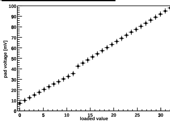
Chip Z36459A-W06-X04-Y10 preamp DAC
