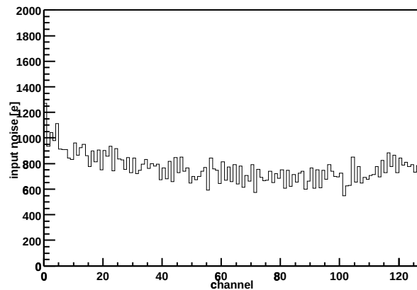
Chip Z36459A-W06-X04-Y10 Input noise vs. channel
