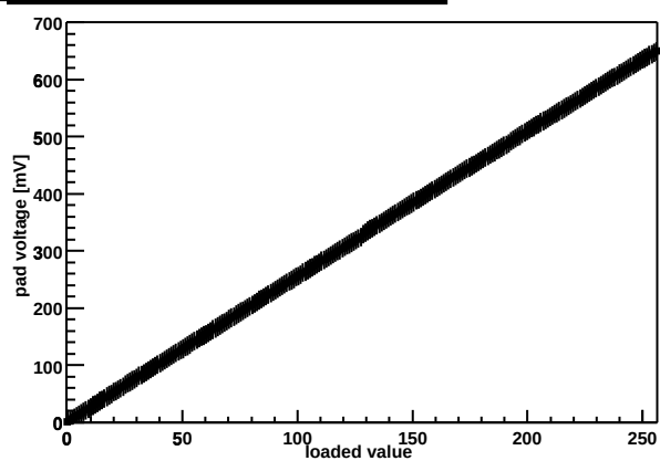
Chip Z36459A-W06-X04-Y10 threshold DAC
