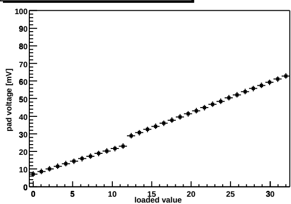
Chip Z36459A-W06-X04-Y10 shaper DAC
