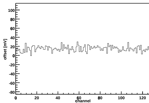
Chip Z36459A-W06-X04-Y10 Offset vs. channel
