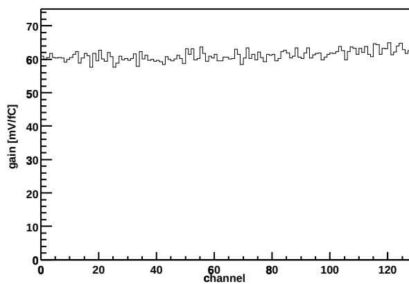
Chip Z36459A-W06-X04-Y10 Gain vs. channel
