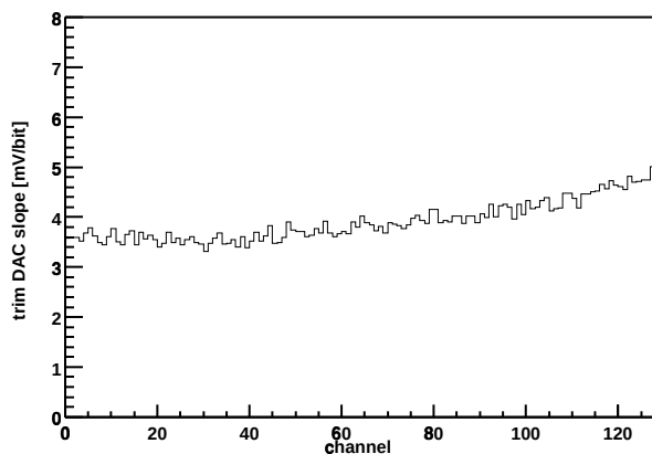
Chip Z36459A-W06-X04-Y10 Trim DAC slope vs. channel
