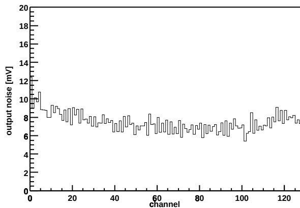
Chip Z36459A-W06-X04-Y10 Output noise vs. channel
