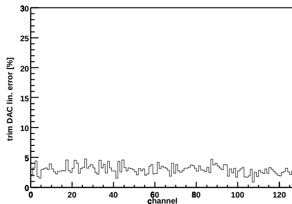
Chip Z36459A-W06-X04-Y10 trim DAC lin. error
