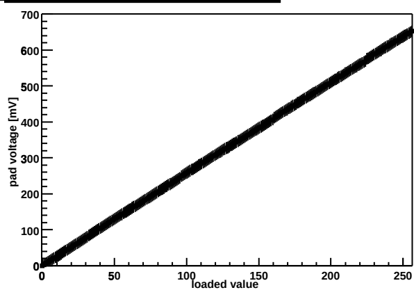
Chip Z36459A-W06-X04-Y16 threshold DAC
