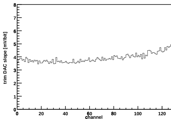
Chip Z36459A-W06-X04-Y16 Trim DAC slope vs. channel
