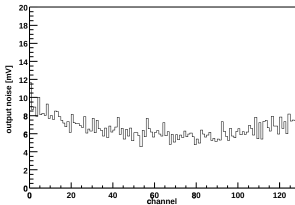
Chip Z36459A-W06-X04-Y16 Output noise vs. channel
