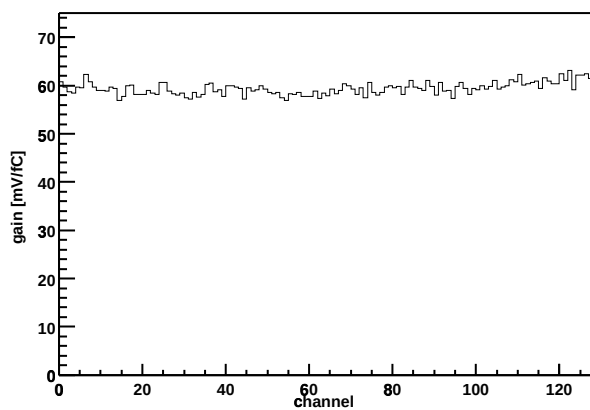
Chip Z36459A-W06-X04-Y16 Gain vs. channel
