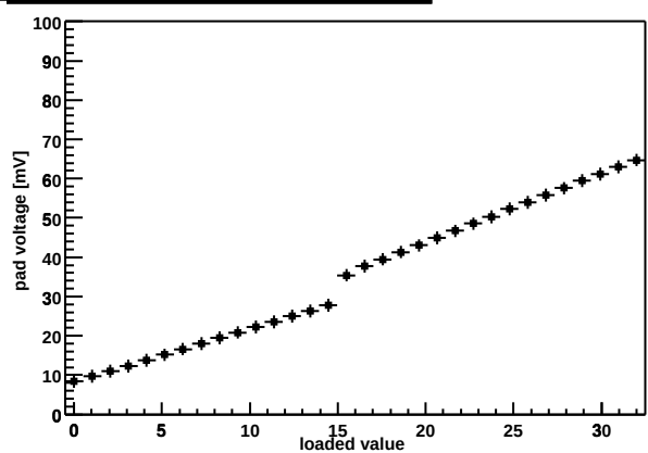
Chip Z36459A-W06-X04-Y16 shaper DAC
