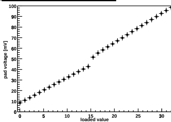
Chip Z36459A-W06-X04-Y16 preamp DAC
