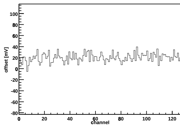
Chip Z36459A-W06-X04-Y16 Offset vs. channel
