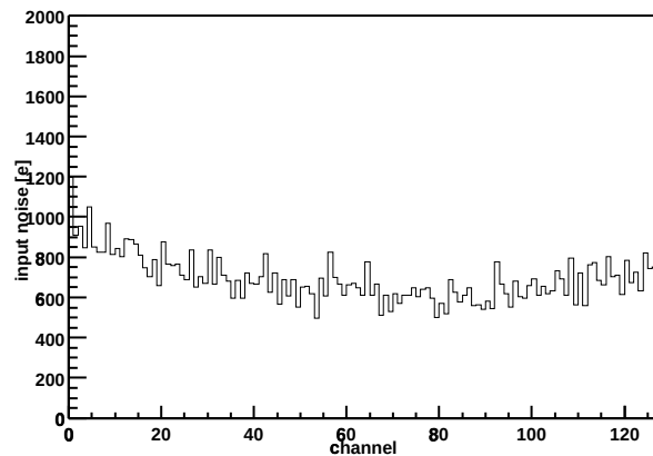
Chip Z36459A-W06-X04-Y16 Input noise vs. channel
