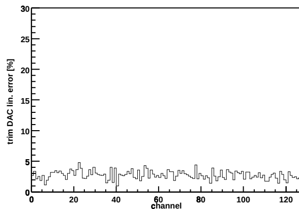
Chip Z36459A-W06-X04-Y16 trim DAC lin. error
