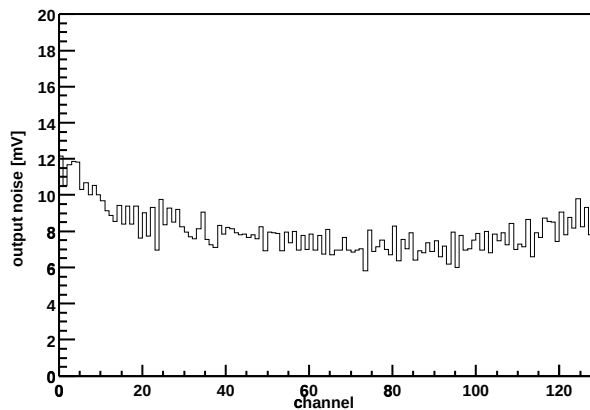
Chip Z36459A-W06-X05-Y05 Output noise vs. channel
