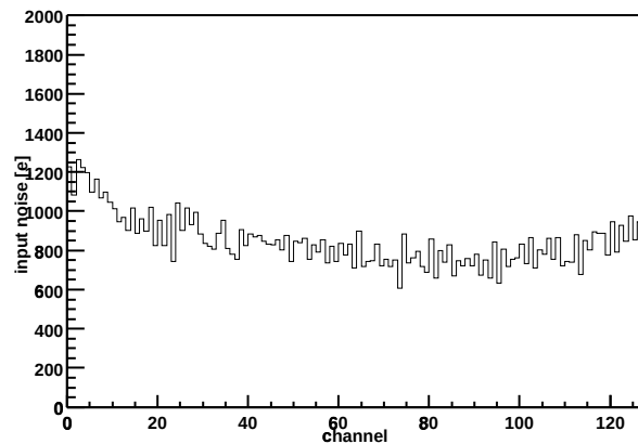
Chip Z36459A-W06-X05-Y05 Input noise vs. channel
