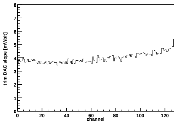
Chip Z36459A-W06-X05-Y05 Trim DAC slope vs. channel
