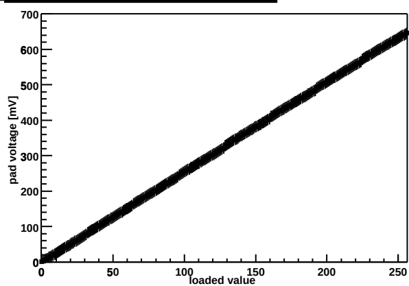
Chip Z36459A-W06-X05-Y05 threshold DAC
