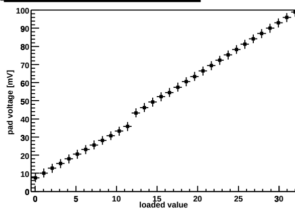
Chip Z36459A-W06-X05-Y05 preamp DAC
