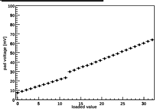
Chip Z36459A-W06-X05-Y05 shaper DAC
