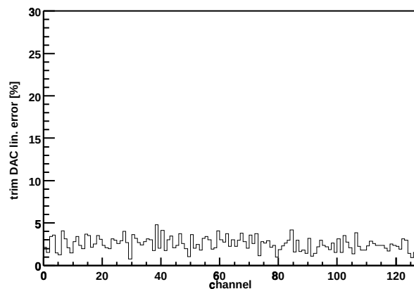
Chip Z36459A-W06-X05-Y05 trim DAC lin. error
