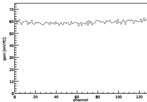
Chip Z36459A-W06-X05-Y05 Gain vs. channel
