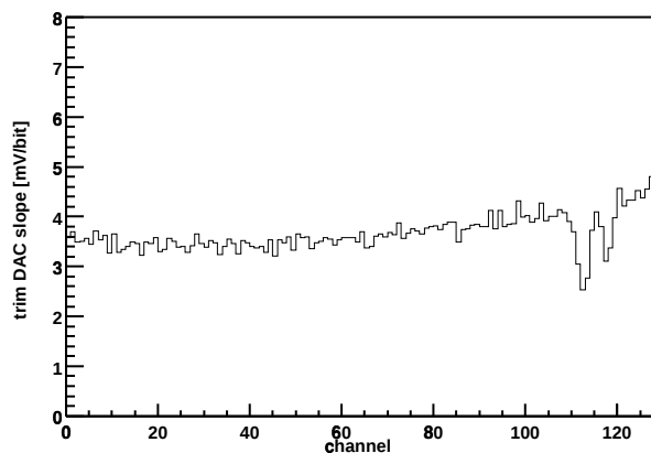
Chip Z36459A-W06-X05-Y17 Trim DAC slope vs. channel
