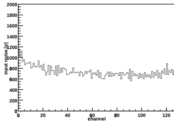
Chip Z36459A-W06-X05-Y17 Input noise vs. channel
