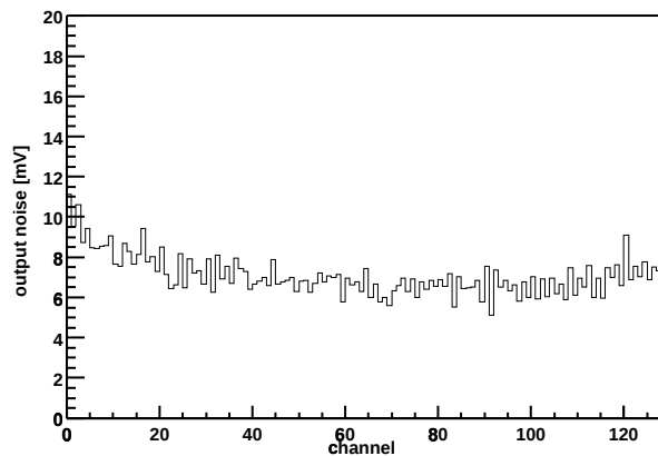
Chip Z36459A-W06-X05-Y17 Output noise vs. channel
