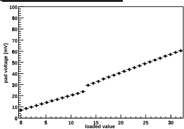
Chip Z36459A-W06-X05-Y17 shaper DAC
