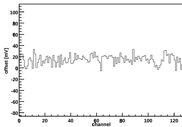
Chip Z36459A-W06-X05-Y17 Offset vs. channel
