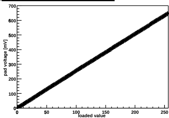
Chip Z36459A-W06-X05-Y17 threshold DAC
