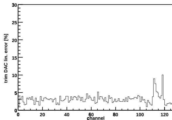
Chip Z36459A-W06-X05-Y17 trim DAC lin. error
