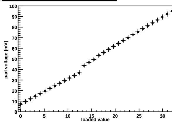
Chip Z36459A-W06-X05-Y17 preamp DAC
