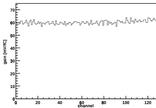
Chip Z36459A-W06-X05-Y17 Gain vs. channel
