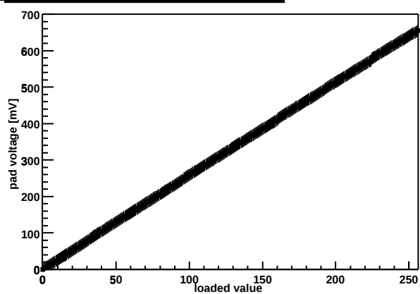
Chip Z36459A-W06-X06-Y05 threshold DAC
