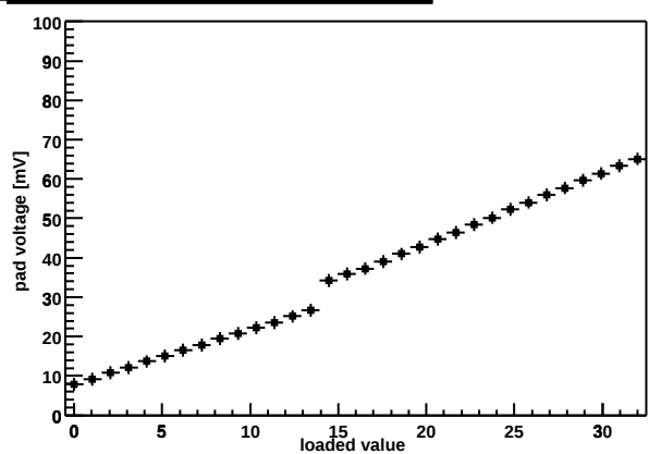
Chip Z36459A-W06-X06-Y05 shaper DAC
