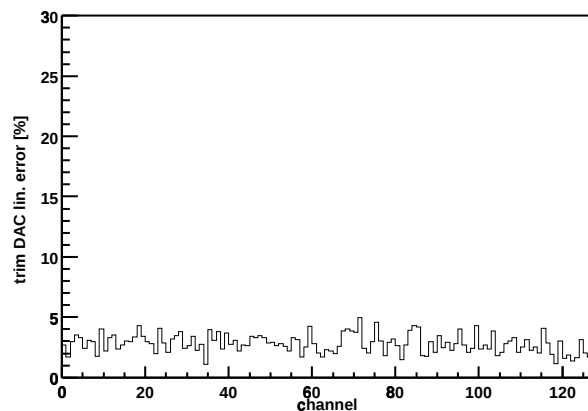
Chip Z36459A-W06-X06-Y05 trim DAC lin. error
