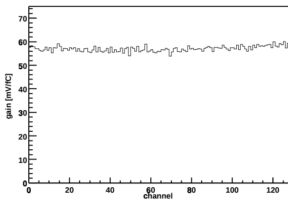
Chip Z36459A-W06-X06-Y05 Gain vs. channel
