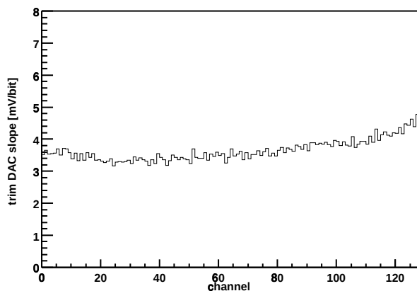
Chip Z36459A-W06-X06-Y05 Trim DAC slope vs. channel
