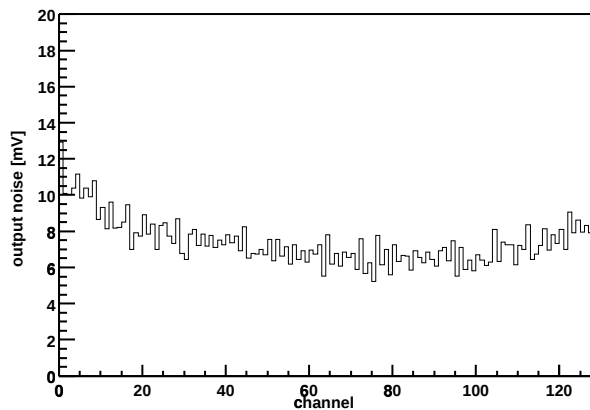
Chip Z36459A-W06-X06-Y05 Output noise vs. channel
