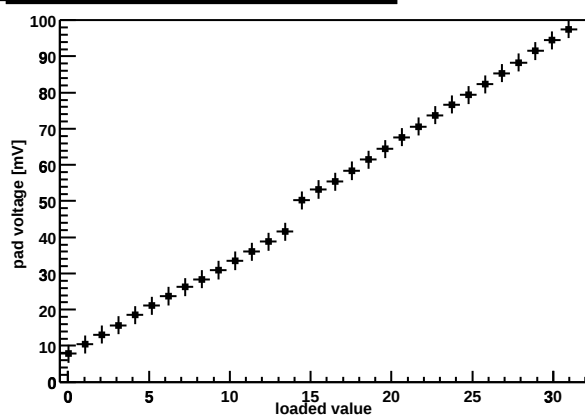
Chip Z36459A-W06-X06-Y05 preamp DAC
