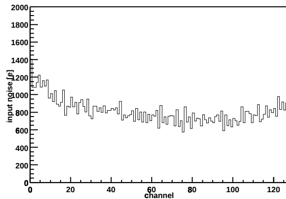
Chip Z36459A-W06-X06-Y05 Input noise vs. channel
