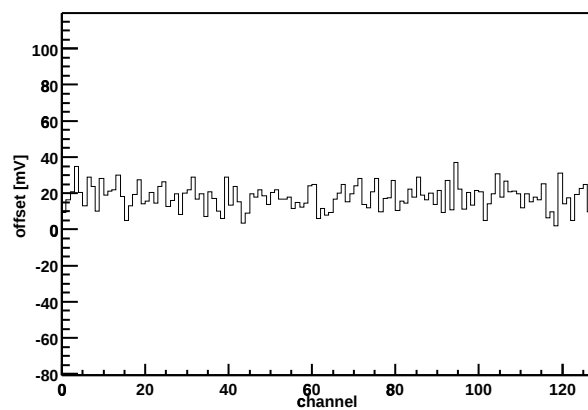
Chip Z36459A-W06-X06-Y05 Offset vs. channel
