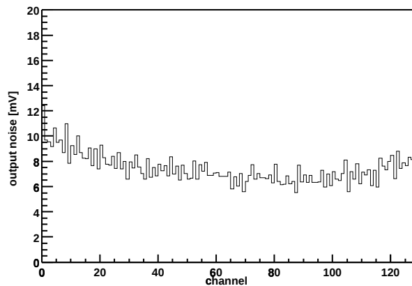
Chip Z36459A-W06-X06-Y12 Output noise vs. channel
