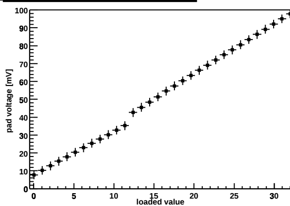
Chip Z36459A-W06-X06-Y12 preamp DAC
