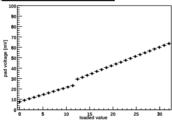
Chip Z36459A-W06-X06-Y12 shaper DAC
