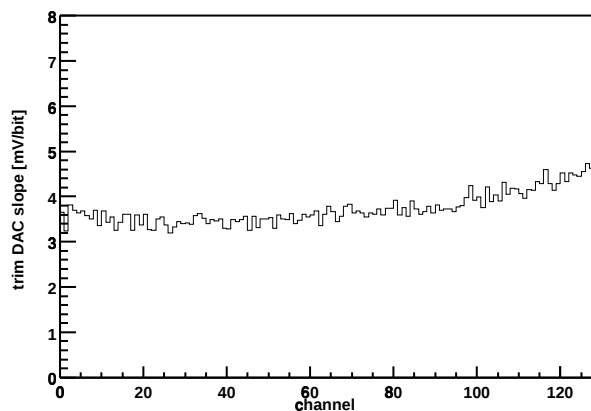
Chip Z36459A-W06-X06-Y12 Trim DAC slope vs. channel
