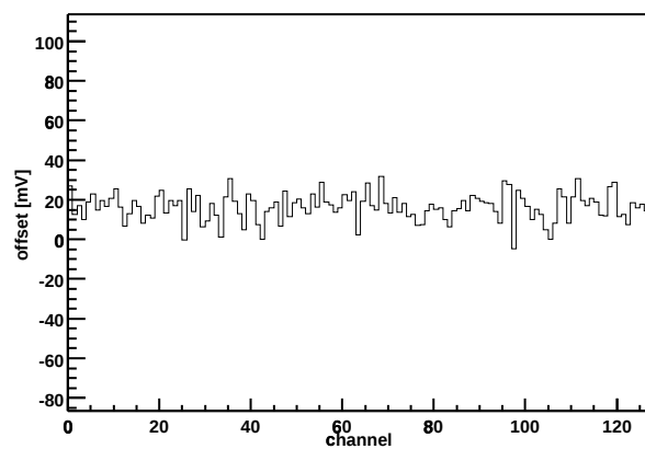
Chip Z36459A-W06-X06-Y12 Offset vs. channel
