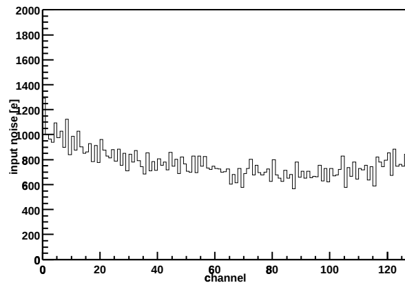
Chip Z36459A-W06-X06-Y12 Input noise vs. channel
