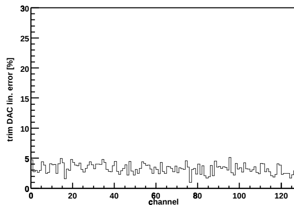
Chip Z36459A-W06-X06-Y12 trim DAC lin. error
