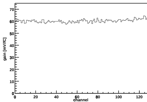
Chip Z36459A-W06-X06-Y12 Gain vs. channel
