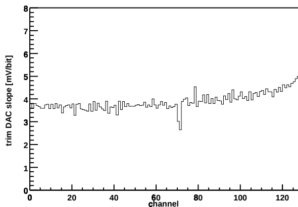
Chip Z36459A-W06-X06-Y18 Trim DAC slope vs. channel
