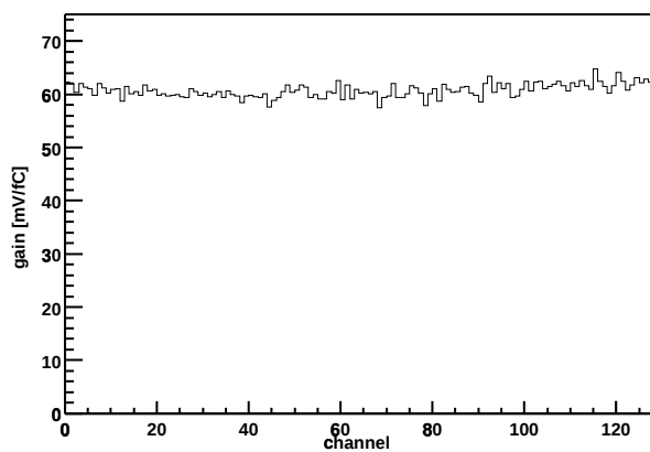
Chip Z36459A-W06-X06-Y18 Gain vs. channel
