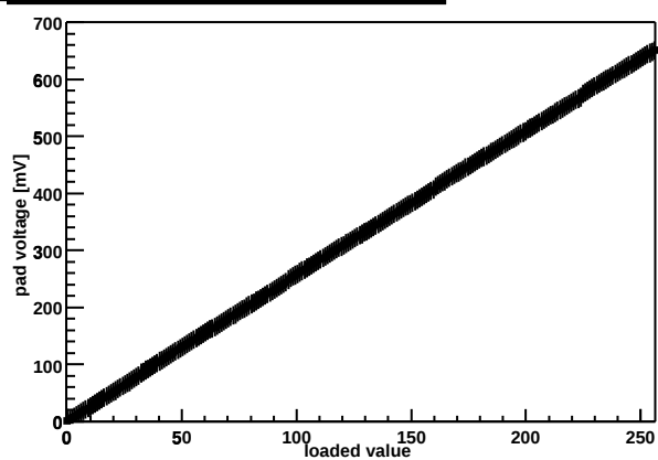
Chip Z36459A-W06-X06-Y18 threshold DAC
