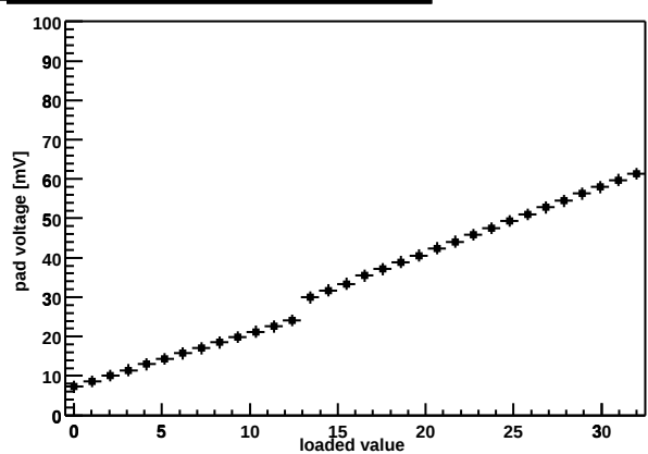
Chip Z36459A-W06-X06-Y18 shaper DAC
