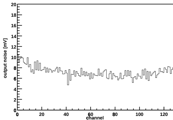
Chip Z36459A-W06-X06-Y18 Output noise vs. channel
