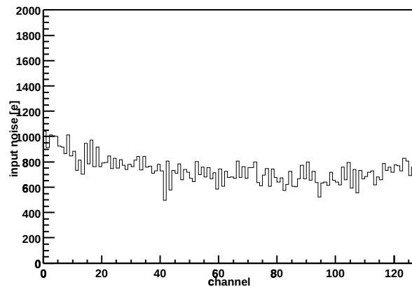
Chip Z36459A-W06-X06-Y18 Input noise vs. channel
