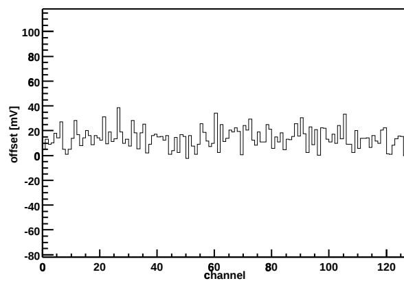
Chip Z36459A-W06-X06-Y18 Offset vs. channel
