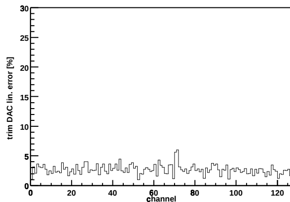
Chip Z36459A-W06-X06-Y18 trim DAC lin. error
