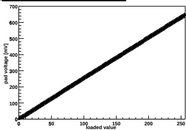
Chip Z36459A-W06-X07-Y04 threshold DAC
