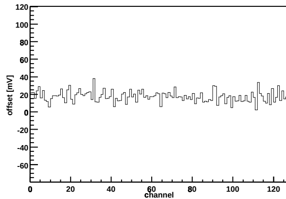
Chip Z36459A-W06-X07-Y04 Offset vs. channel
