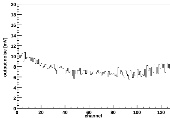
Chip Z36459A-W06-X07-Y04 Output noise vs. channel
