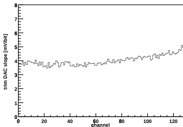
Chip Z36459A-W06-X07-Y04 Trim DAC slope vs. channel
