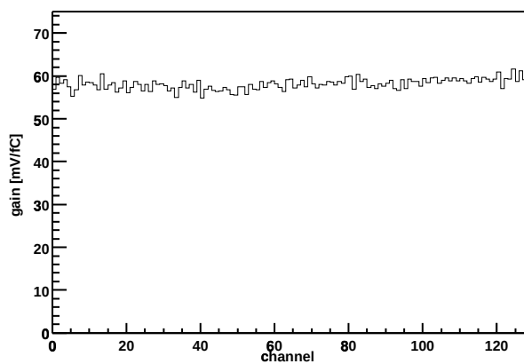
Chip Z36459A-W06-X07-Y04 Gain vs. channel
