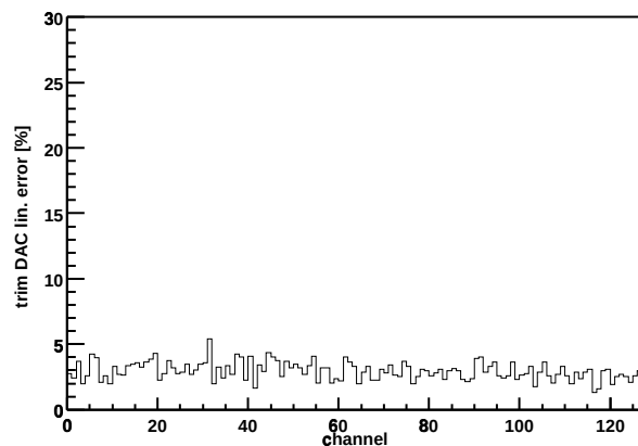
Chip Z36459A-W06-X07-Y04 trim DAC lin. error
