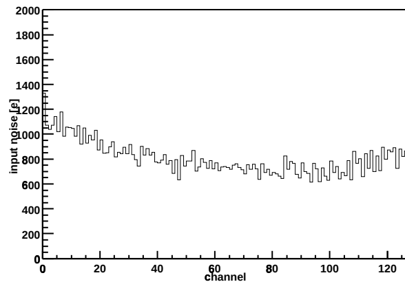
Chip Z36459A-W06-X07-Y04 Input noise vs. channel
