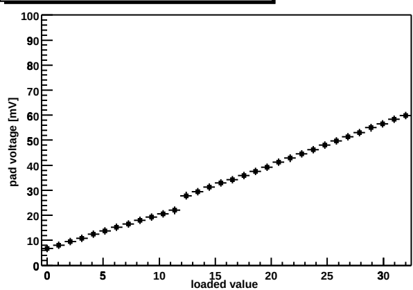
Chip Z36459A-W06-X07-Y07 shaper DAC
