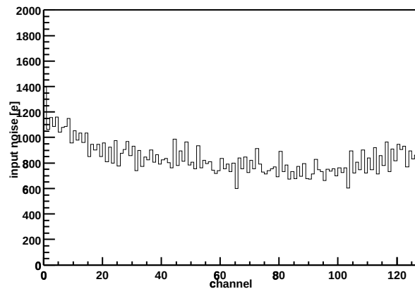
Chip Z36459A-W06-X07-Y07 Input noise vs. channel
