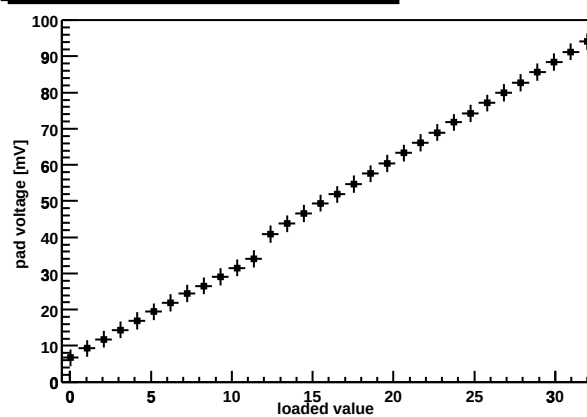
Chip Z36459A-W06-X07-Y07 preamp DAC
