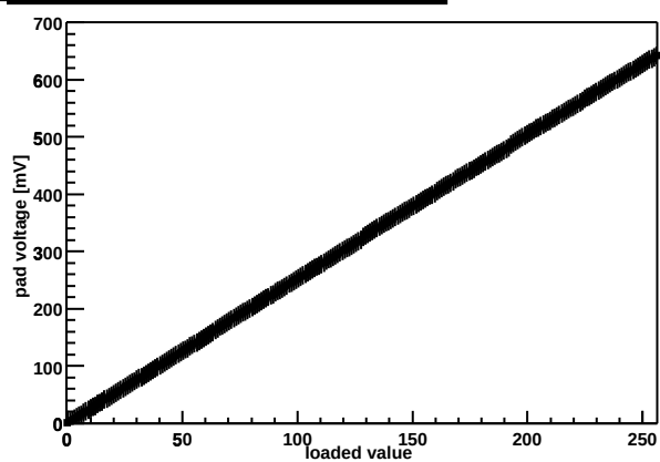
Chip Z36459A-W06-X07-Y07 threshold DAC
