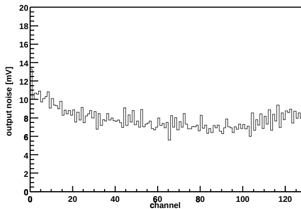
Chip Z36459A-W06-X07-Y07 Output noise vs. channel
