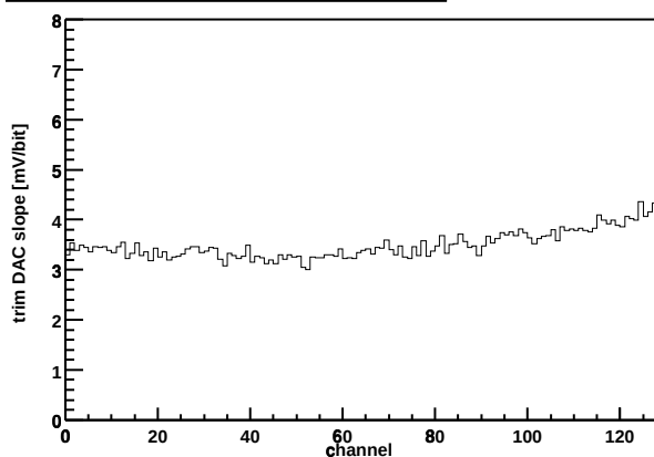
Chip Z36459A-W06-X07-Y07 Trim DAC slope vs. channel
