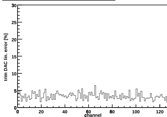
Chip Z36459A-W06-X07-Y07 trim DAC lin. error
