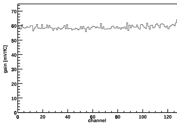
Chip Z36459A-W06-X07-Y07 Gain vs. channel
