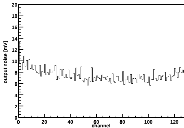
Chip Z36459A-W06-X07-Y12 Output noise vs. channel
