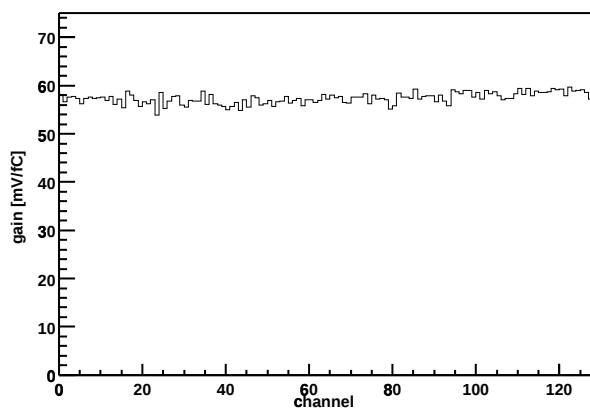
Chip Z36459A-W06-X07-Y12 Gain vs. channel
