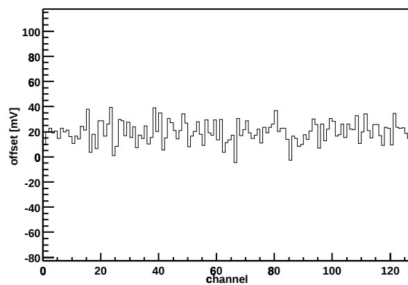
Chip Z36459A-W06-X07-Y12 Offset vs. channel
