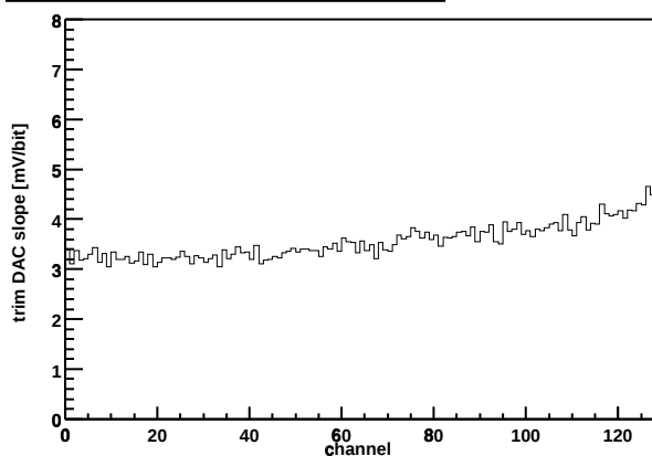
Chip Z36459A-W06-X07-Y12 Trim DAC slope vs. channel
