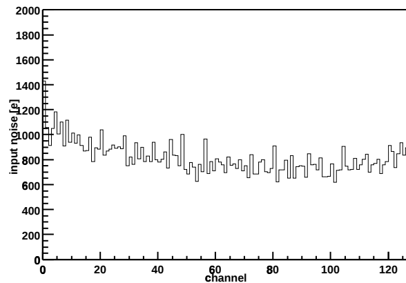
Chip Z36459A-W06-X07-Y12 Input noise vs. channel
