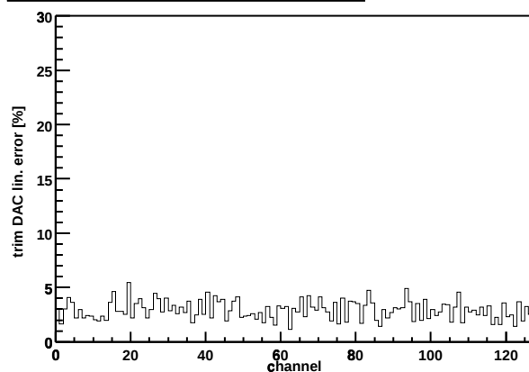
Chip Z36459A-W06-X07-Y12 trim DAC lin. error
