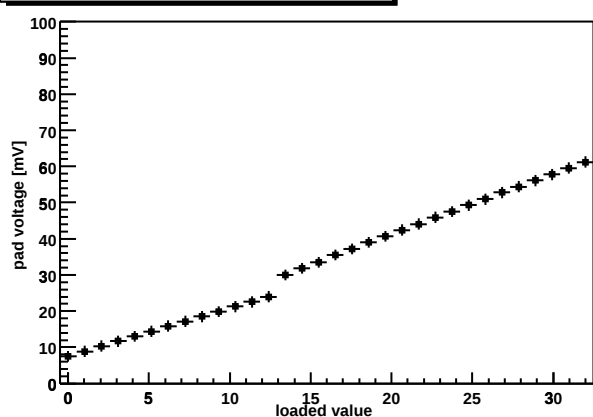
Chip Z36459A-W06-X07-Y12 shaper DAC
