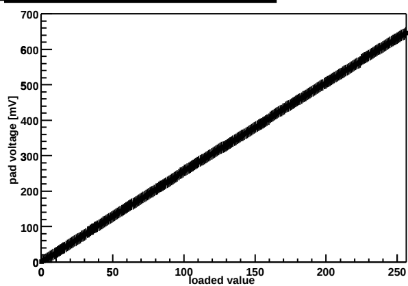
Chip Z36459A-W06-X07-Y12 threshold DAC
