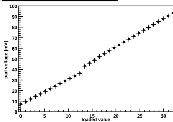
Chip Z36459A-W06-X07-Y15 preamp DAC
