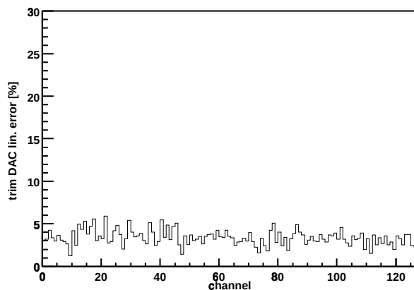
Chip Z36459A-W06-X07-Y15 trim DAC lin. error
