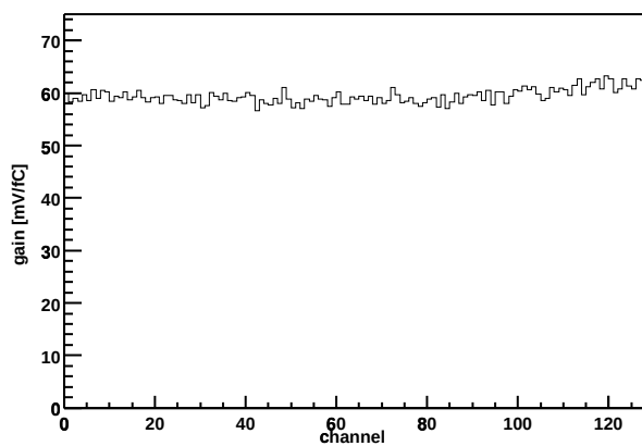
Chip Z36459A-W06-X07-Y15 Gain vs. channel
