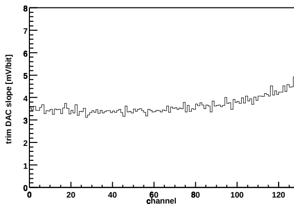
Chip Z36459A-W06-X07-Y15 Trim DAC slope vs. channel
