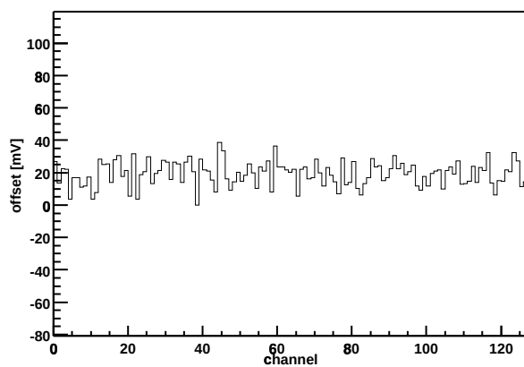
Chip Z36459A-W06-X07-Y15 Offset vs. channel
