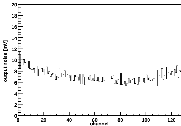
Chip Z36459A-W06-X07-Y15 Output noise vs. channel
