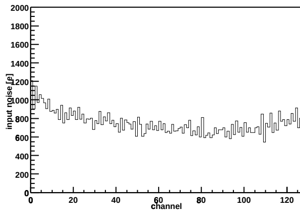
Chip Z36459A-W06-X07-Y15 Input noise vs. channel
