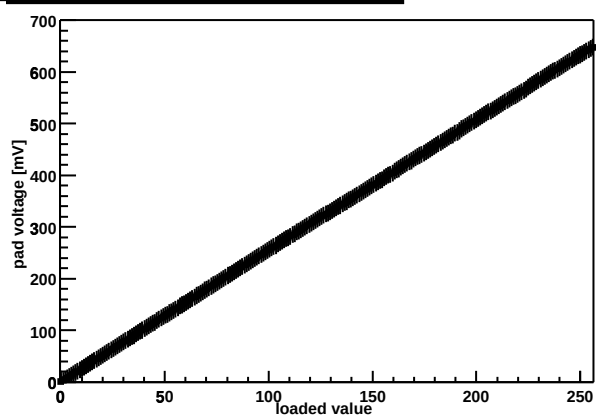
Chip Z36459A-W06-X07-Y15 threshold DAC
