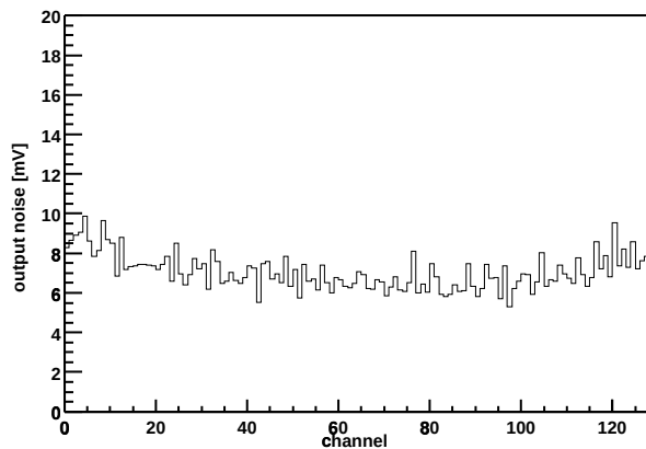
Chip Z36459A-W06-X07-Y17 Output noise vs. channel
