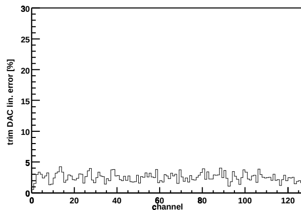
Chip Z36459A-W06-X07-Y17 trim DAC lin. error
