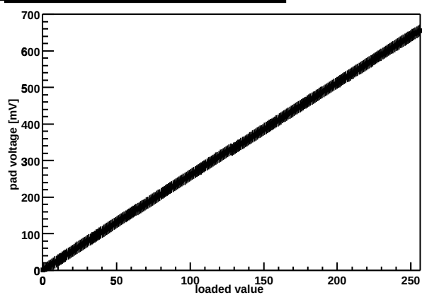
Chip Z36459A-W06-X07-Y17 threshold DAC
