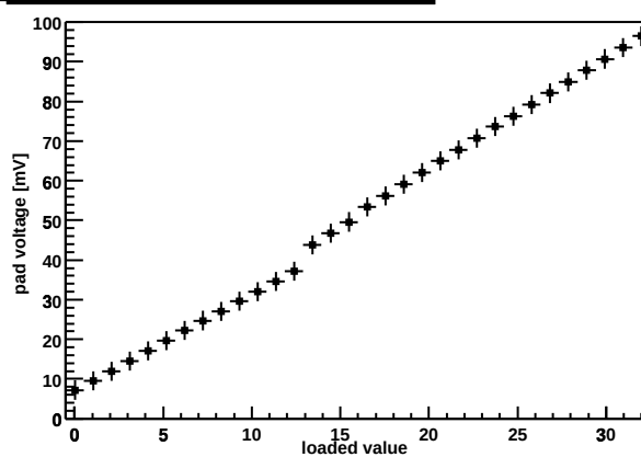
Chip Z36459A-W06-X07-Y17 preamp DAC
