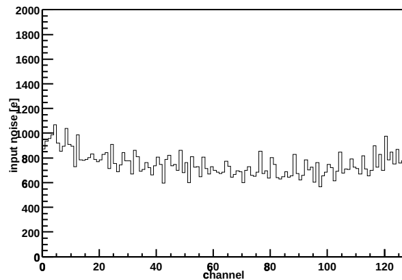
Chip Z36459A-W06-X07-Y17 Input noise vs. channel
