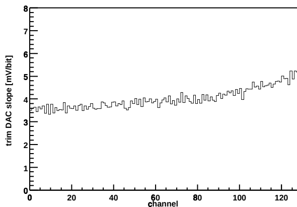
Chip Z36459A-W06-X07-Y17 Trim DAC slope vs. channel
