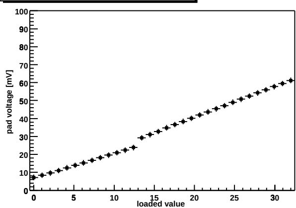
Chip Z36459A-W06-X07-Y17 shaper DAC
