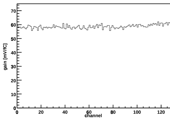
Chip Z36459A-W06-X07-Y17 Gain vs. channel
