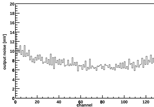
Chip Z36459A-W06-X08-Y02 Output noise vs. channel
