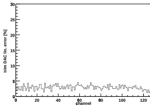
Chip Z36459A-W06-X08-Y02 trim DAC lin. error
