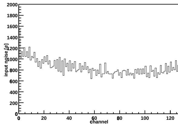
Chip Z36459A-W06-X08-Y02 Input noise vs. channel
