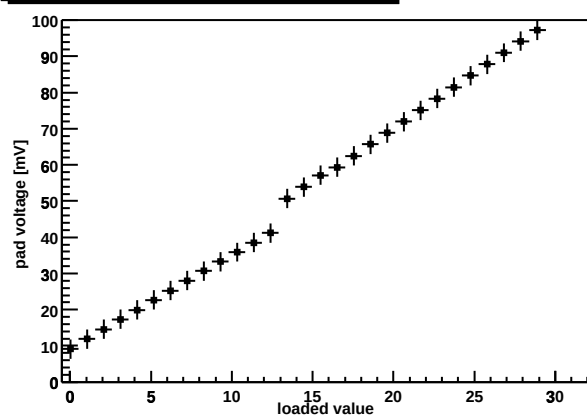
Chip Z36459A-W06-X08-Y02 preamp DAC
