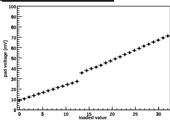
Chip Z36459A-W06-X08-Y02 shaper DAC
