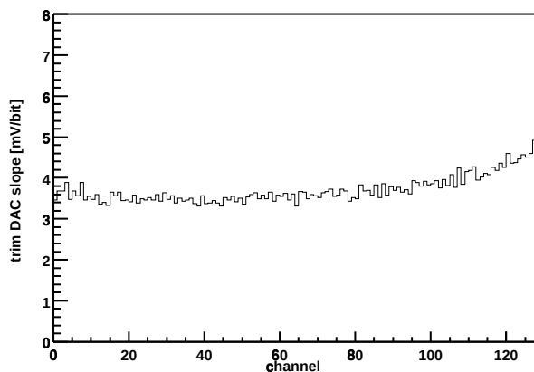
Chip Z36459A-W06-X08-Y02 Trim DAC slope vs. channel
