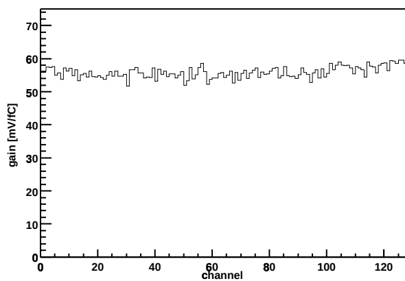
Chip Z36459A-W06-X08-Y02 Gain vs. channel
