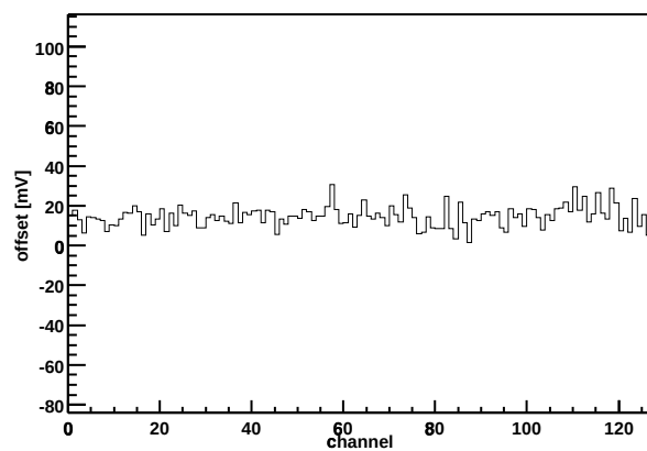
Chip Z36459A-W06-X08-Y02 Offset vs. channel
