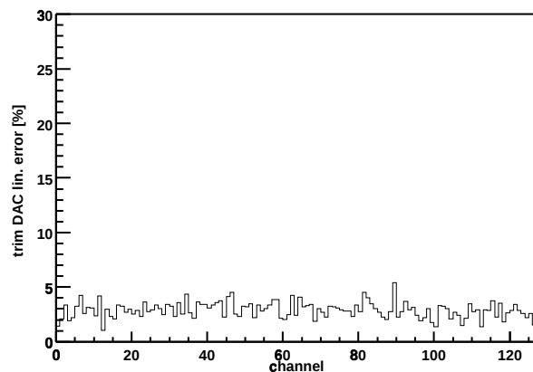
Chip Z36459A-W06-X08-Y03 trim DAC lin. error
