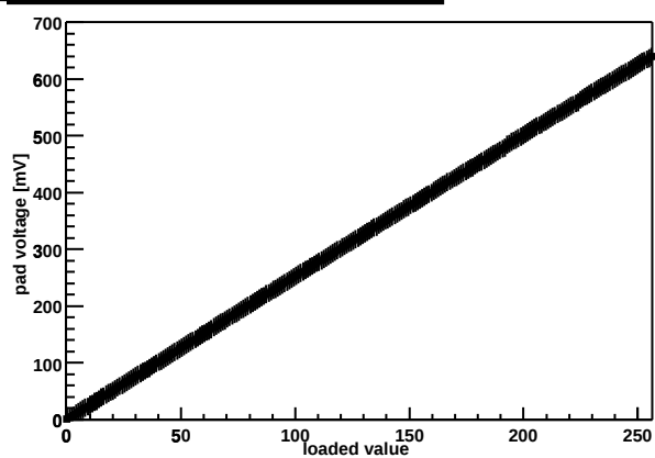
Chip Z36459A-W06-X08-Y03 threshold DAC
