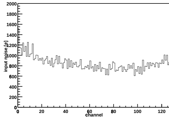
Chip Z36459A-W06-X08-Y03 Input noise vs. channel
