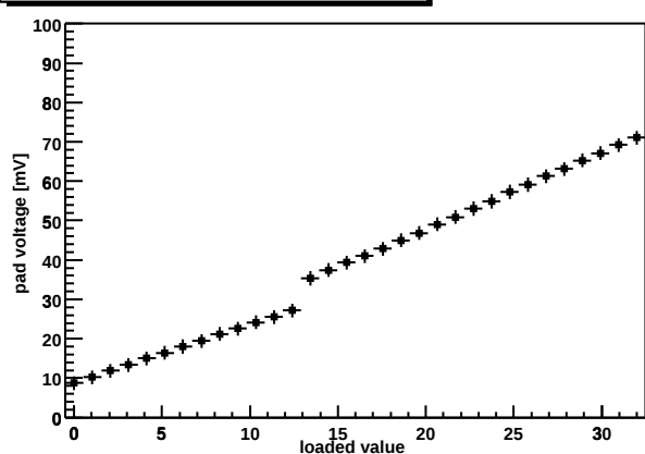
Chip Z36459A-W06-X08-Y03 shaper DAC
