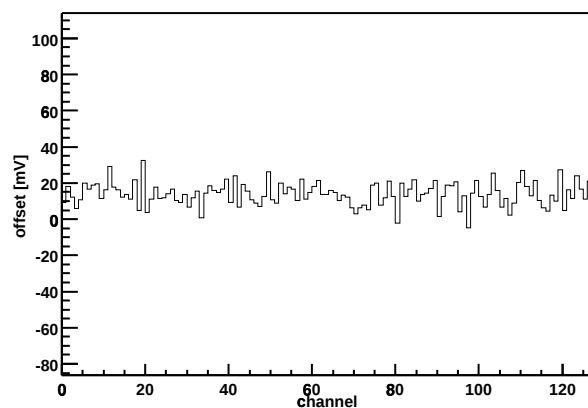
Chip Z36459A-W06-X08-Y03 Offset vs. channel
