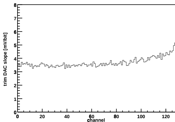
Chip Z36459A-W06-X08-Y03 Trim DAC slope vs. channel
