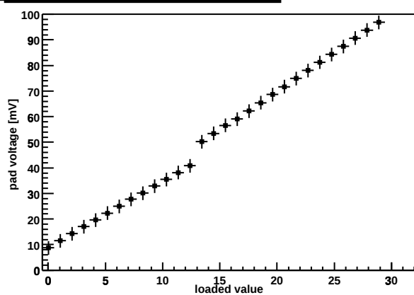
Chip Z36459A-W06-X08-Y03 preamp DAC
