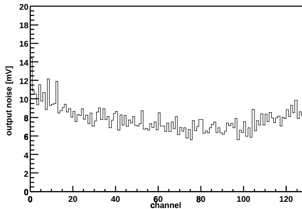
Chip Z36459A-W06-X08-Y03 Output noise vs. channel
