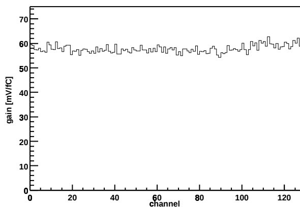
Chip Z36459A-W06-X08-Y03 Gain vs. channel
