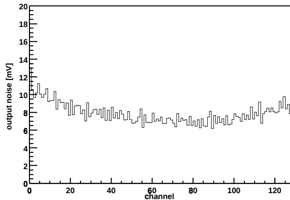
Chip Z36459A-W06-X08-Y07 Output noise vs. channel
