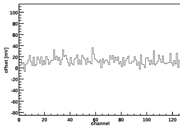
Chip Z36459A-W06-X08-Y07 Offset vs. channel
