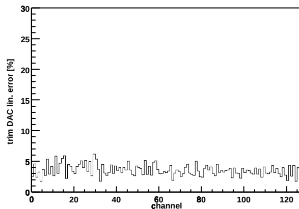
Chip Z36459A-W06-X08-Y07 trim DAC lin. error
