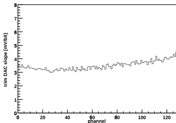
Chip Z36459A-W06-X08-Y07 Trim DAC slope vs. channel
