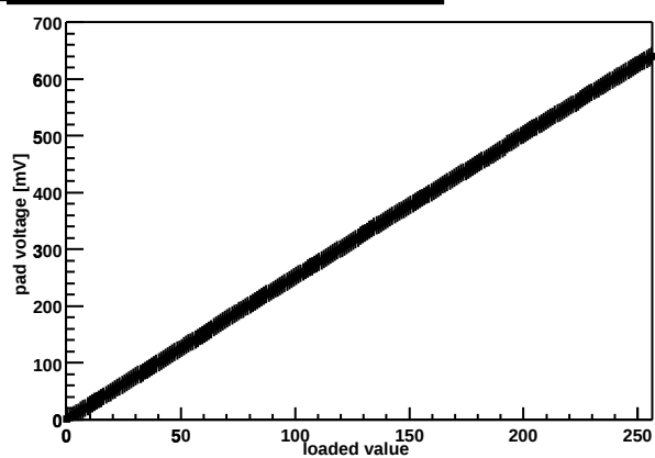
Chip Z36459A-W06-X08-Y07 threshold DAC
