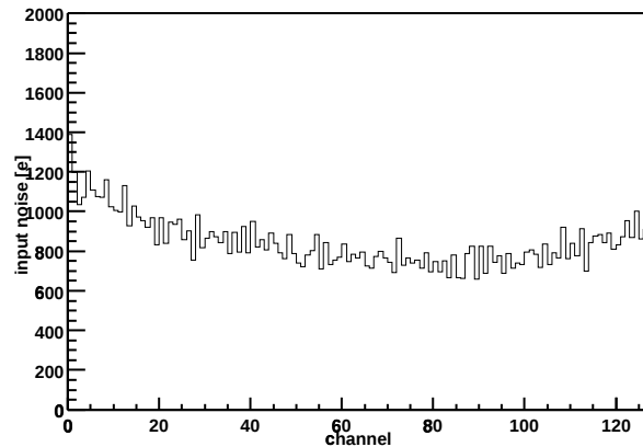
Chip Z36459A-W06-X08-Y07 Input noise vs. channel
