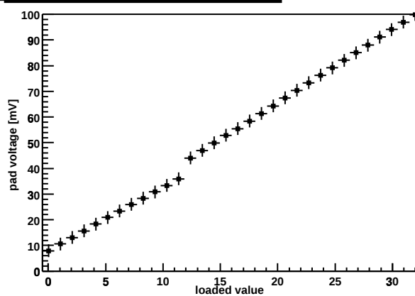
Chip Z36459A-W06-X08-Y07 preamp DAC
