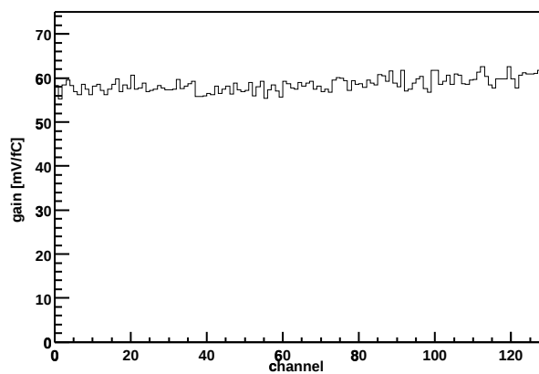
Chip Z36459A-W06-X08-Y07 Gain vs. channel
