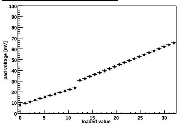
Chip Z36459A-W06-X08-Y07 shaper DAC
