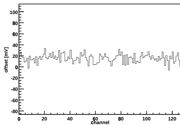
Chip Z36459A-W06-X08-Y10 Offset vs. channel
