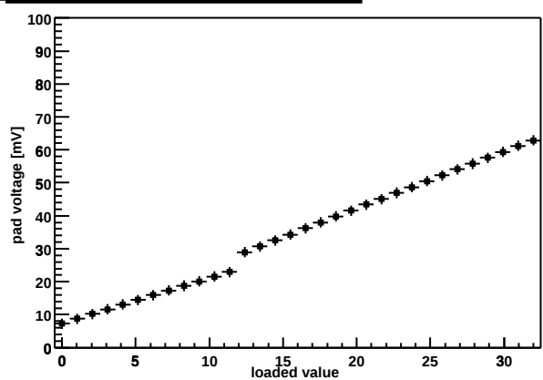
Chip Z36459A-W06-X08-Y10 shaper DAC
