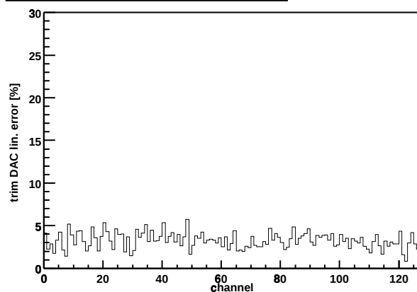
Chip Z36459A-W06-X08-Y10 trim DAC lin. error
