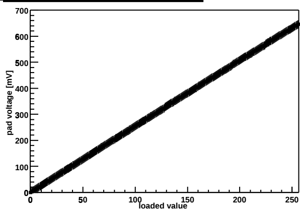
Chip Z36459A-W06-X08-Y10 threshold DAC
