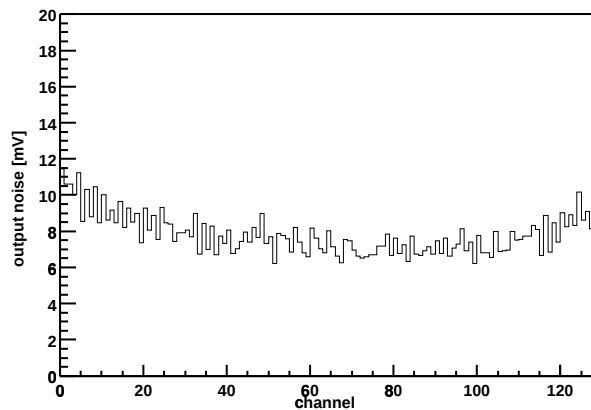
Chip Z36459A-W06-X08-Y10 Output noise vs. channel
