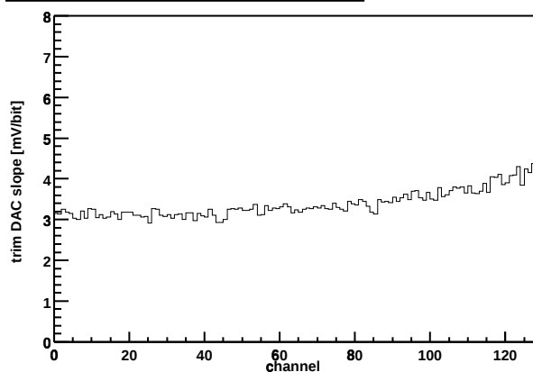
Chip Z36459A-W06-X08-Y10 Trim DAC slope vs. channel
