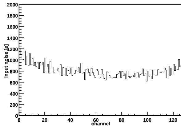
Chip Z36459A-W06-X08-Y10 Input noise vs. channel
