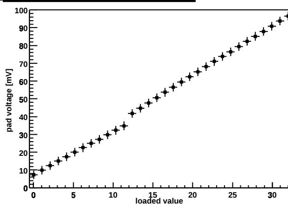
Chip Z36459A-W06-X08-Y10 preamp DAC
