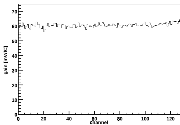
Chip Z36459A-W06-X08-Y10 Gain vs. channel
