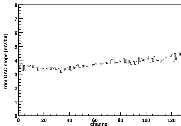
Chip Z36459A-W06-X08-Y17 Trim DAC slope vs. channel
