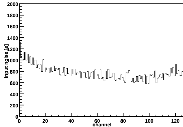
Chip Z36459A-W06-X08-Y17 Input noise vs. channel
