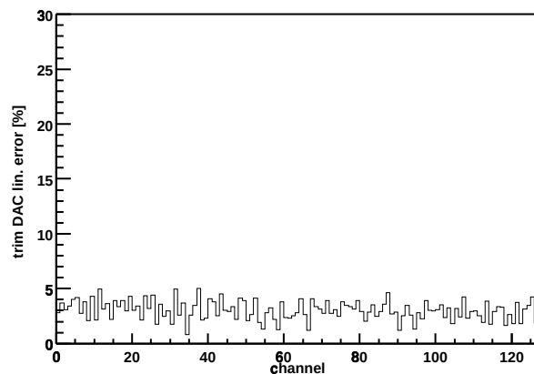
Chip Z36459A-W06-X08-Y17 trim DAC lin. error
