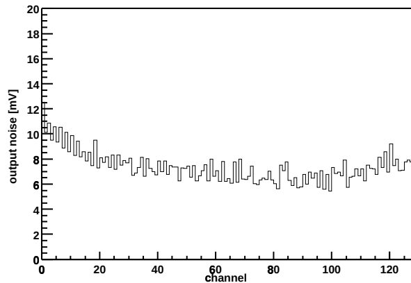
Chip Z36459A-W06-X08-Y17 Output noise vs. channel
