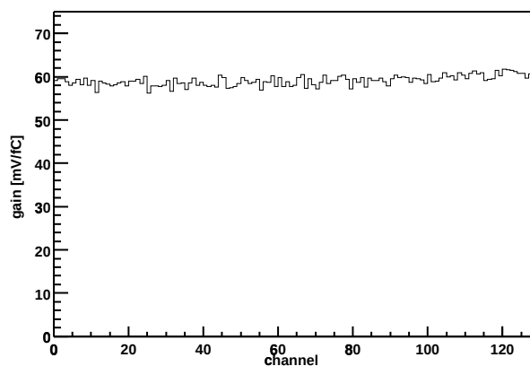
Chip Z36459A-W06-X08-Y17 Gain vs. channel
