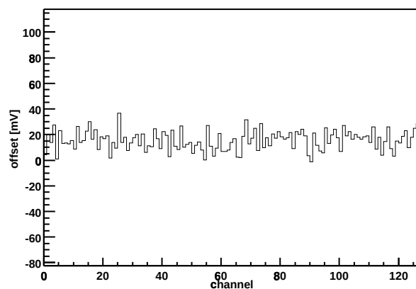
Chip Z36459A-W06-X08-Y17 Offset vs. channel
