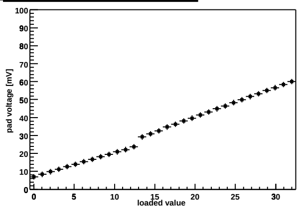
Chip Z36459A-W06-X08-Y17 shaper DAC
