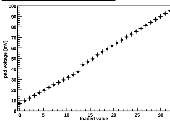
Chip Z36459A-W06-X08-Y17 preamp DAC
