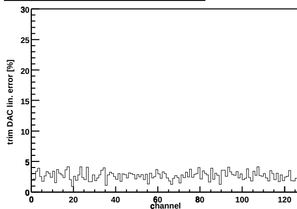
Chip Z36459A-W06-X08-Y18 trim DAC lin. error
