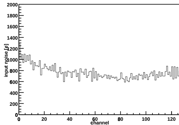
Chip Z36459A-W06-X08-Y18 Input noise vs. channel
