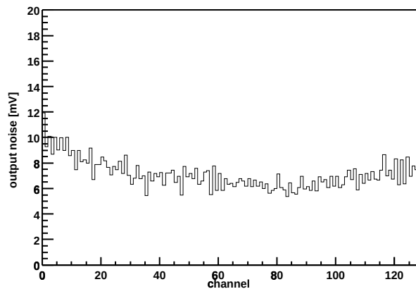
Chip Z36459A-W06-X08-Y18 Output noise vs. channel
