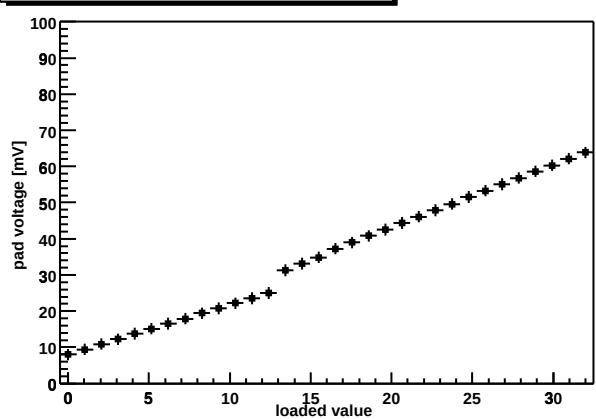
Chip Z36459A-W06-X08-Y18 shaper DAC
