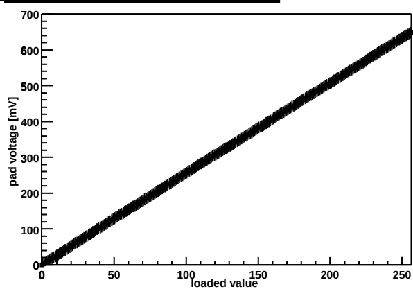
Chip Z36459A-W06-X08-Y18 threshold DAC
