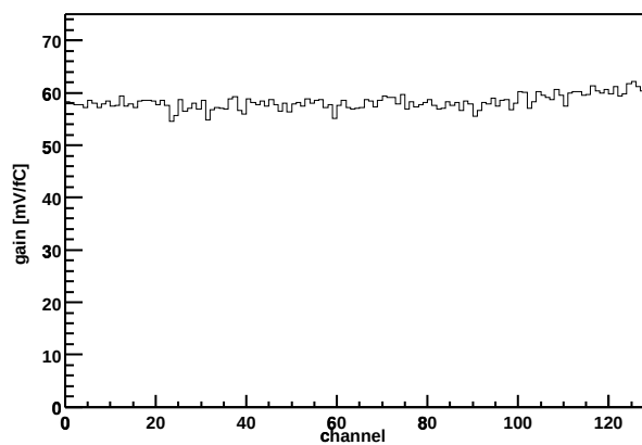
Chip Z36459A-W06-X08-Y18 Gain vs. channel
