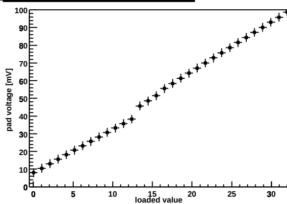
Chip Z36459A-W06-X08-Y18 preamp DAC
