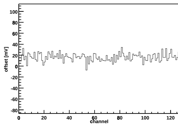
Chip Z36459A-W06-X08-Y18 Offset vs. channel
