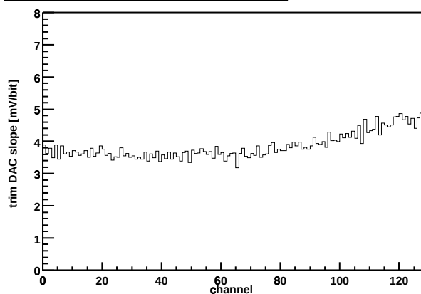
Chip Z36459A-W06-X08-Y18 Trim DAC slope vs. channel
