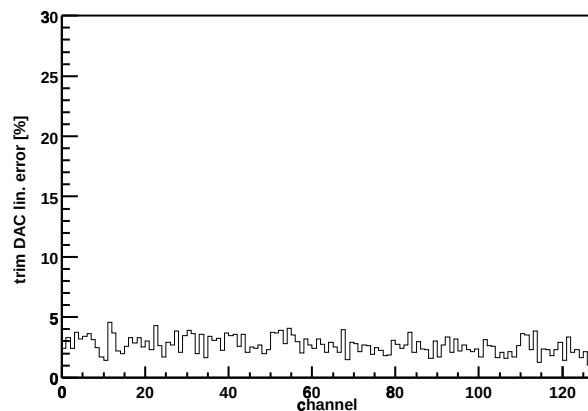
Chip Z36459A-W06-X09-Y04 trim DAC lin. error
