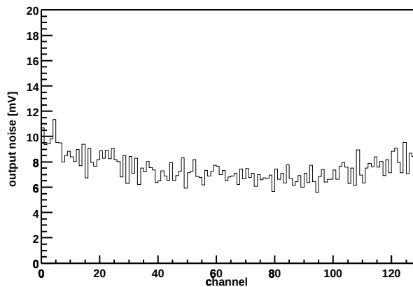
Chip Z36459A-W06-X09-Y04 Output noise vs. channel
