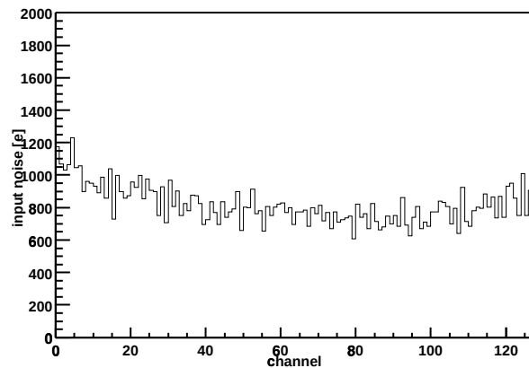
Chip Z36459A-W06-X09-Y04 Input noise vs. channel
