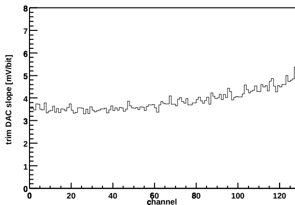
Chip Z36459A-W06-X09-Y04 Trim DAC slope vs. channel
