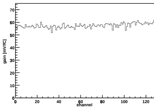
Chip Z36459A-W06-X09-Y04 Gain vs. channel
