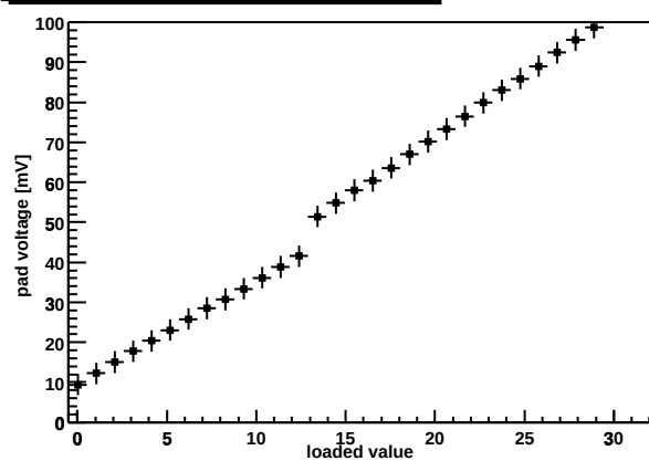
Chip Z36459A-W06-X09-Y04 preamp DAC
