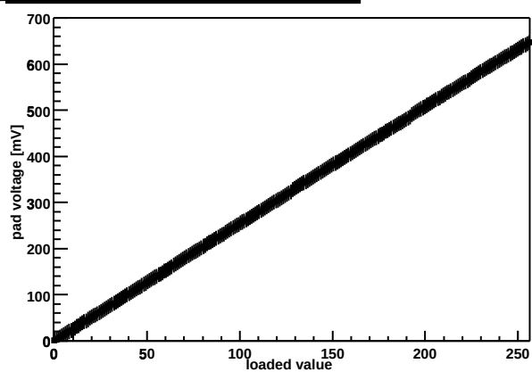
Chip Z36459A-W06-X09-Y04 threshold DAC
