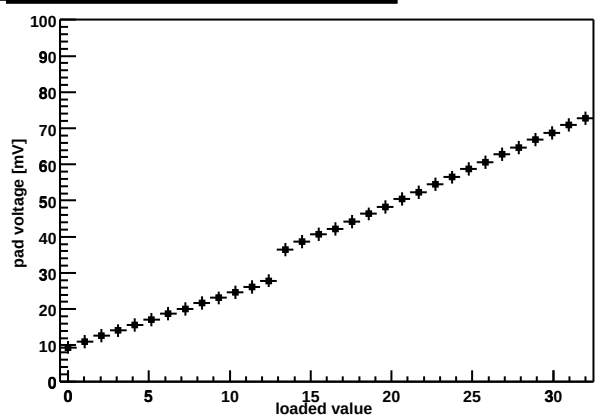
Chip Z36459A-W06-X09-Y04 shaper DAC
