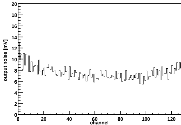
Chip Z36459A-W06-X09-Y05 Output noise vs. channel
