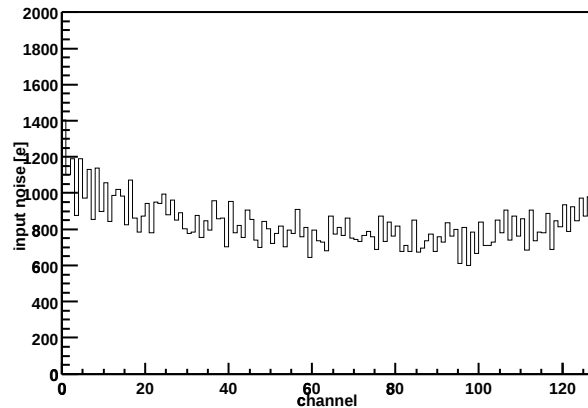
Chip Z36459A-W06-X09-Y05 Input noise vs. channel
