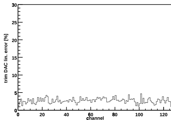
Chip Z36459A-W06-X09-Y05 trim DAC lin. error
