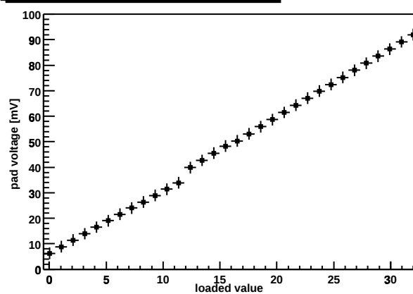
Chip Z36459A-W06-X09-Y05 preamp DAC
