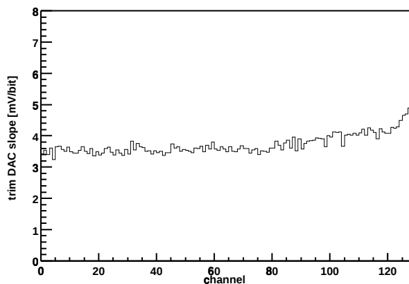
Chip Z36459A-W06-X09-Y05 Trim DAC slope vs. channel
