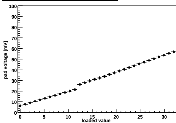
Chip Z36459A-W06-X09-Y05 shaper DAC
