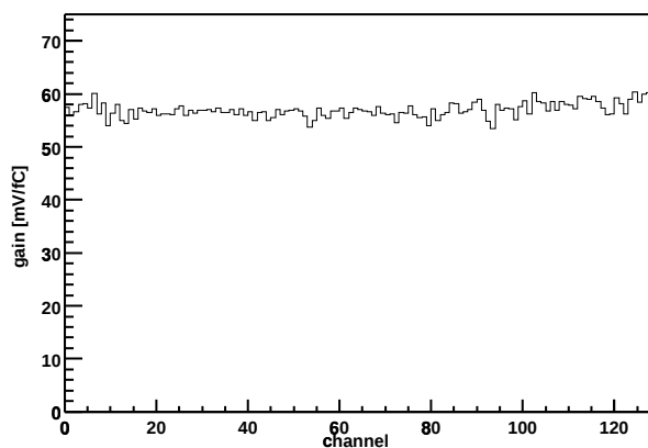
Chip Z36459A-W06-X09-Y05 Gain vs. channel
