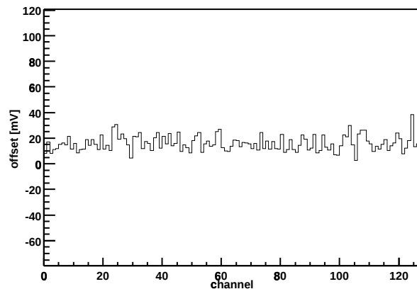
Chip Z36459A-W06-X09-Y05 Offset vs. channel
