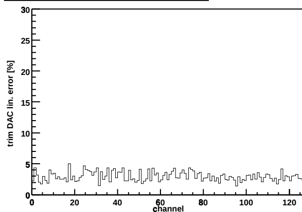
Chip Z36459A-W06-X09-Y12 trim DAC lin. error
