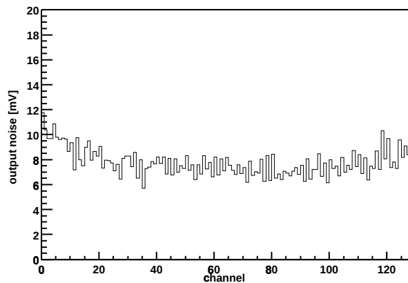
Chip Z36459A-W06-X09-Y12 Output noise vs. channel
