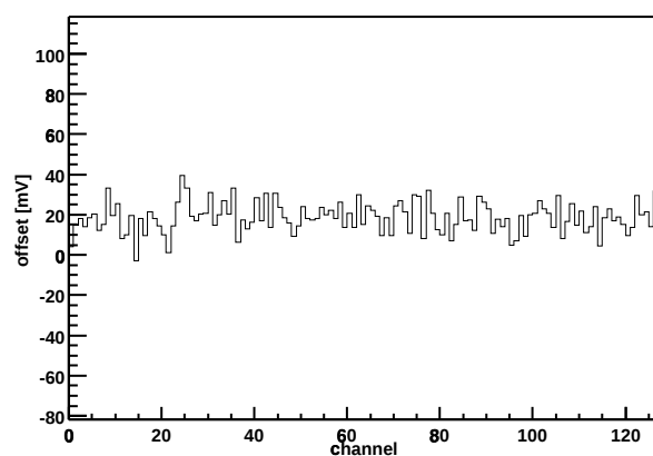
Chip Z36459A-W06-X09-Y12 Offset vs. channel
