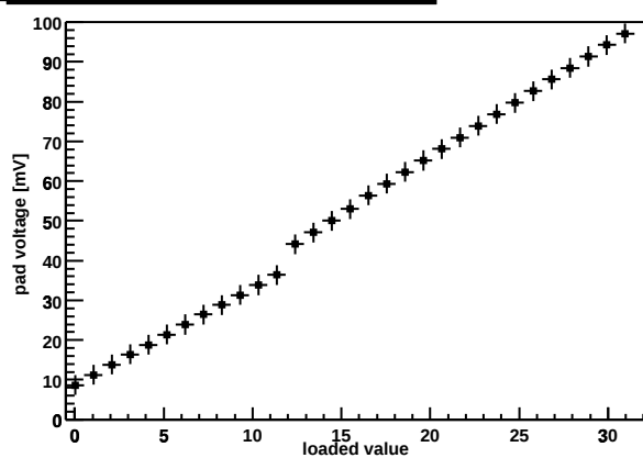
Chip Z36459A-W06-X09-Y12 preamp DAC
