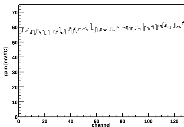
Chip Z36459A-W06-X09-Y12 Gain vs. channel
