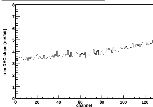
Chip Z36459A-W06-X09-Y12 Trim DAC slope vs. channel
