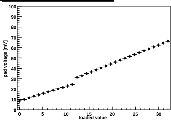
Chip Z36459A-W06-X09-Y12 shaper DAC
