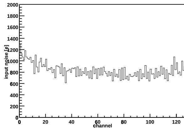
Chip Z36459A-W06-X09-Y12 Input noise vs. channel
