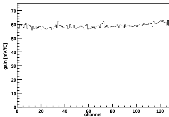
Chip Z36459A-W06-X09-Y13 Gain vs. channel
