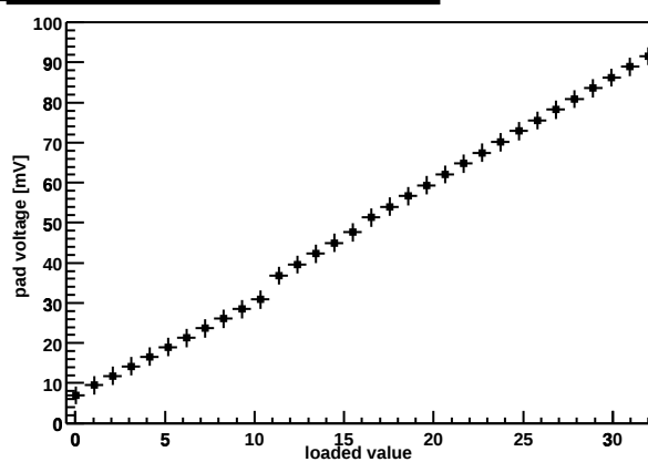
Chip Z36459A-W06-X09-Y13 preamp DAC
