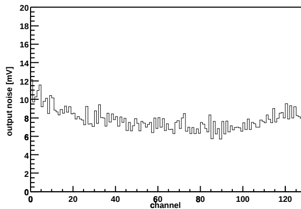
Chip Z36459A-W06-X09-Y13 Output noise vs. channel
