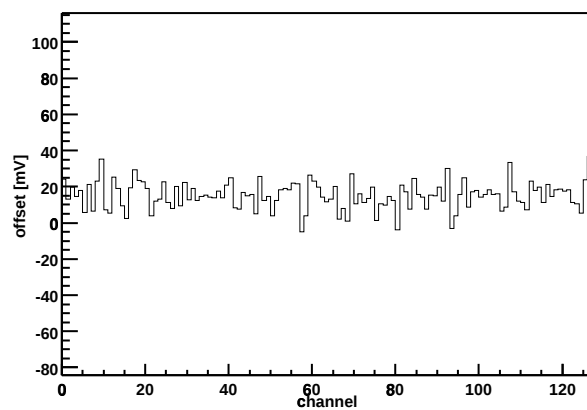
Chip Z36459A-W06-X09-Y13 Offset vs. channel
