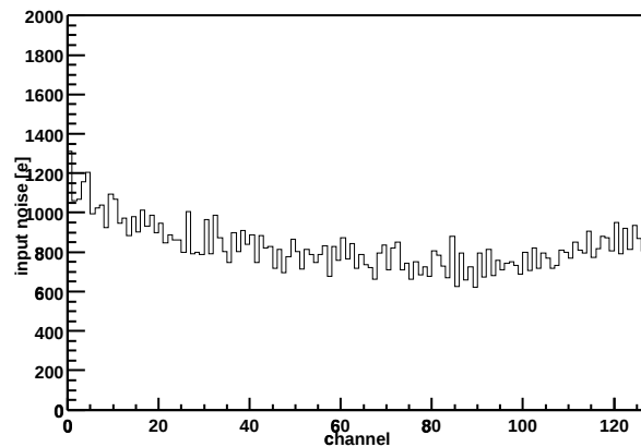
Chip Z36459A-W06-X09-Y13 Input noise vs. channel
