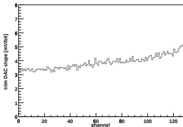
Chip Z36459A-W06-X09-Y13 Trim DAC slope vs. channel
