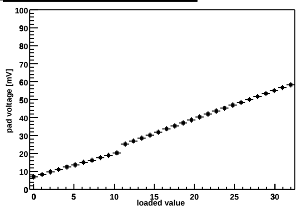
Chip Z36459A-W06-X09-Y13 shaper DAC
