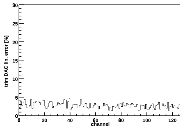
Chip Z36459A-W06-X09-Y13 trim DAC lin. error
