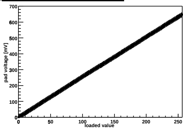
Chip Z36459A-W06-X09-Y13 threshold DAC
