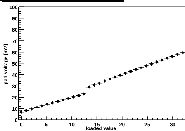
Chip Z36459A-W06-X09-Y14 shaper DAC
