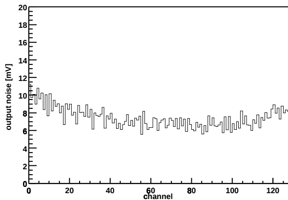
Chip Z36459A-W06-X09-Y14 Output noise vs. channel
