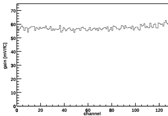
Chip Z36459A-W06-X09-Y14 Gain vs. channel
