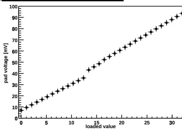
Chip Z36459A-W06-X09-Y14 preamp DAC
