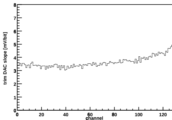
Chip Z36459A-W06-X09-Y14 Trim DAC slope vs. channel
