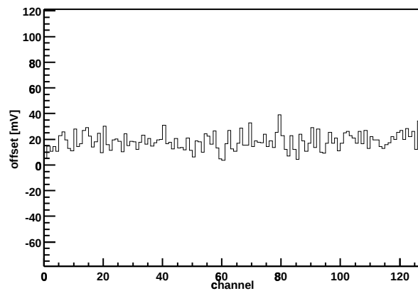
Chip Z36459A-W06-X09-Y14 Offset vs. channel
