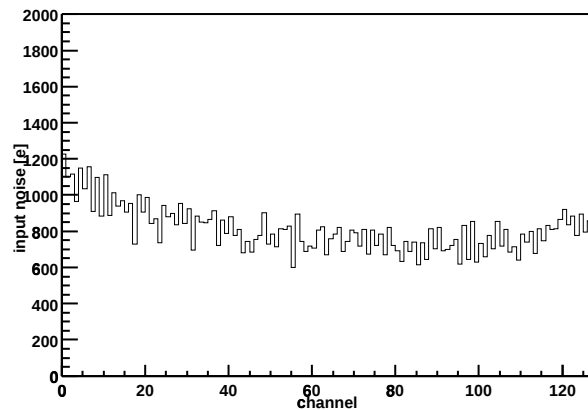
Chip Z36459A-W06-X09-Y14 Input noise vs. channel
