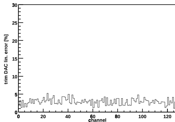
Chip Z36459A-W06-X09-Y14 trim DAC lin. error
