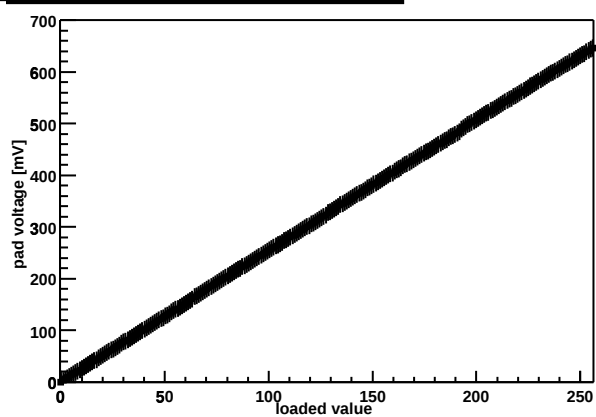
Chip Z36459A-W06-X10-Y06 threshold DAC
