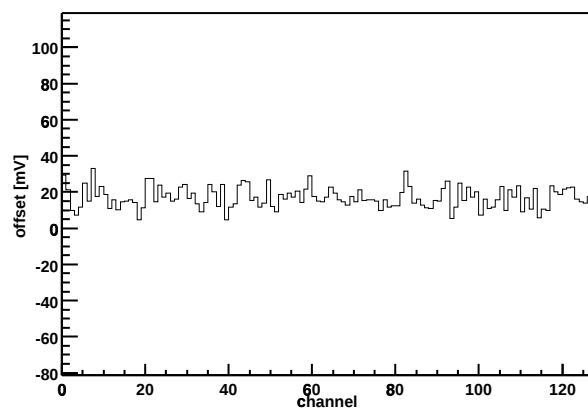
Chip Z36459A-W06-X10-Y06 Offset vs. channel
