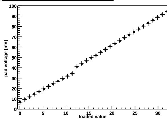
Chip Z36459A-W06-X10-Y06 preamp DAC
