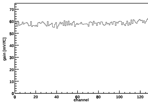
Chip Z36459A-W06-X10-Y06 Gain vs. channel
