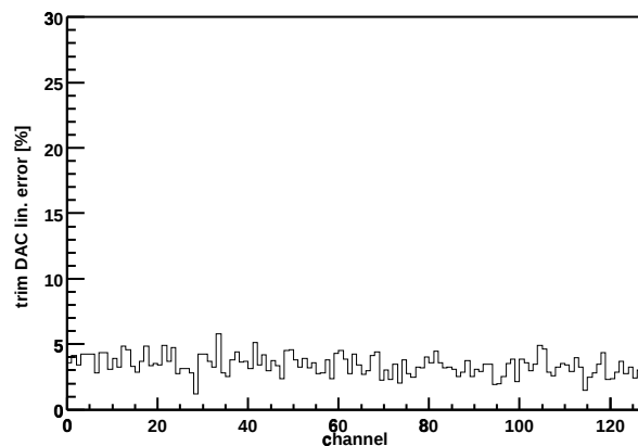
Chip Z36459A-W06-X10-Y06 trim DAC lin. error
