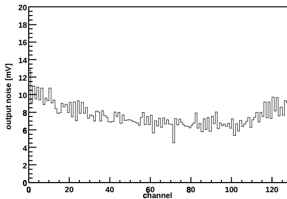
Chip Z36459A-W06-X10-Y06 Output noise vs. channel
