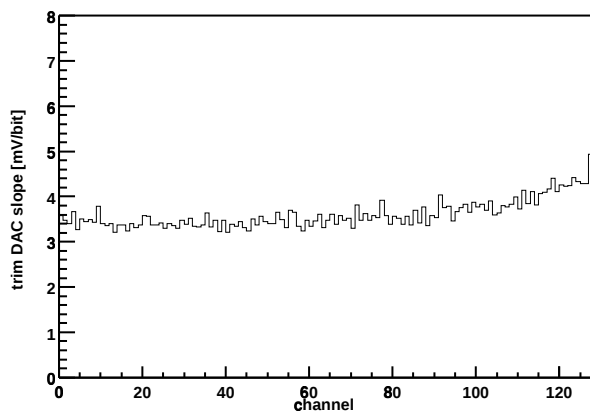
Chip Z36459A-W06-X10-Y06 Trim DAC slope vs. channel
