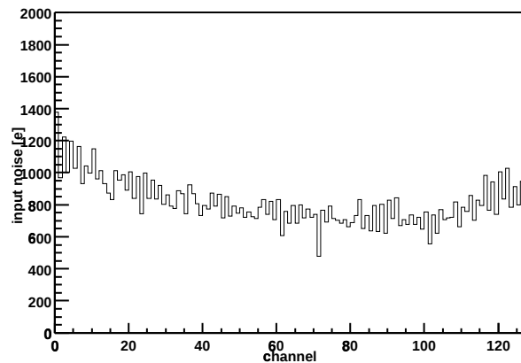
Chip Z36459A-W06-X10-Y06 Input noise vs. channel
