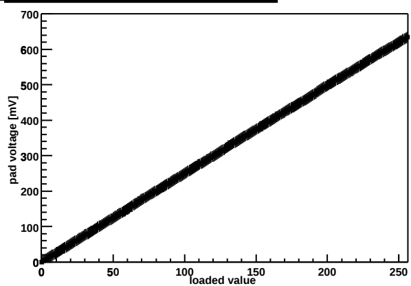
Chip Z36459A-W06-X10-Y09 threshold DAC
