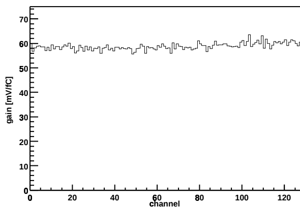
Chip Z36459A-W06-X10-Y09 Gain vs. channel
