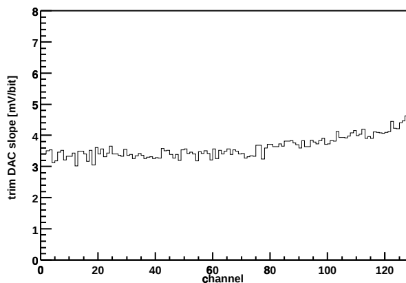
Chip Z36459A-W06-X10-Y09 Trim DAC slope vs. channel
