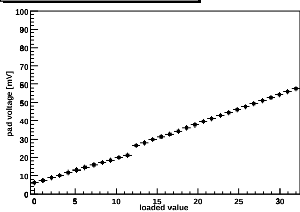
Chip Z36459A-W06-X10-Y09 shaper DAC
