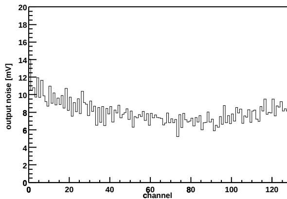
Chip Z36459A-W06-X10-Y09 Output noise vs. channel
