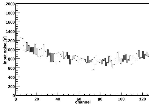
Chip Z36459A-W06-X10-Y09 Input noise vs. channel
