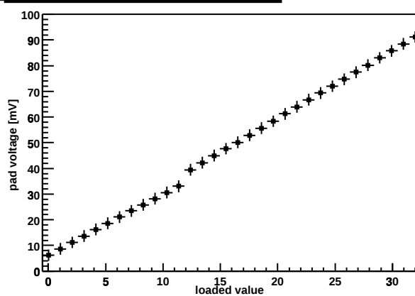
Chip Z36459A-W06-X10-Y09 preamp DAC
