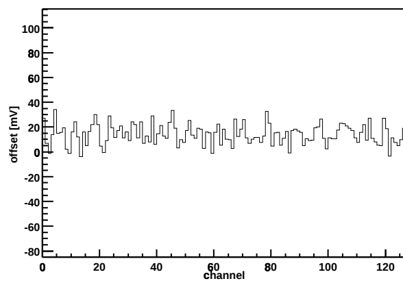
Chip Z36459A-W06-X10-Y09 Offset vs. channel
