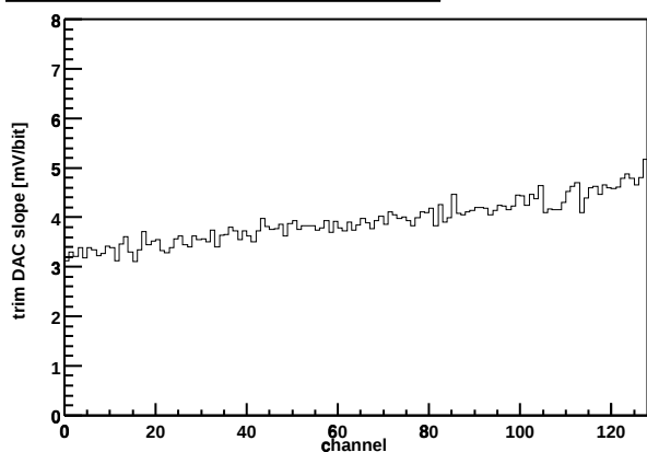
Chip Z36459A-W06-X10-Y10 Trim DAC slope vs. channel
