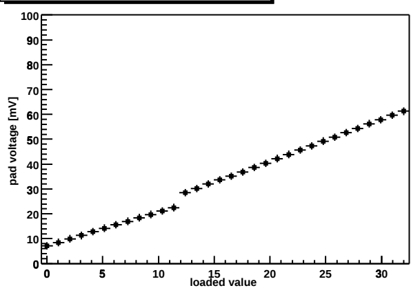
Chip Z36459A-W06-X10-Y10 shaper DAC
