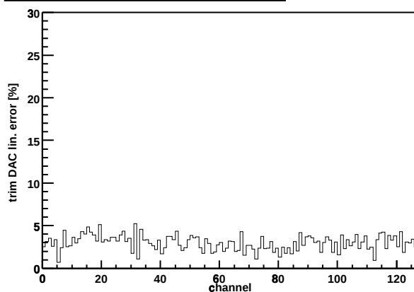
Chip Z36459A-W06-X10-Y10 trim DAC lin. error
