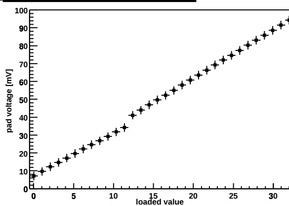
Chip Z36459A-W06-X10-Y10 preamp DAC
