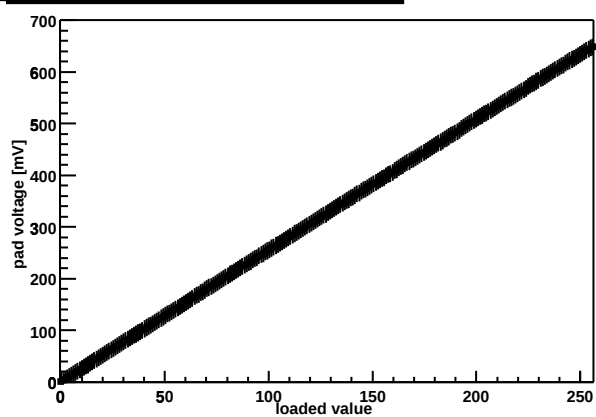
Chip Z36459A-W06-X10-Y10 threshold DAC
