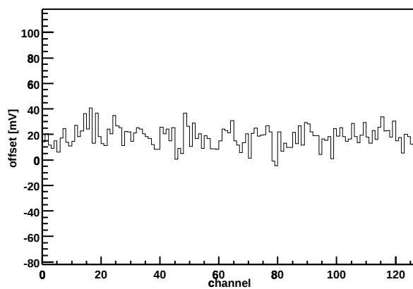
Chip Z36459A-W06-X10-Y10 Offset vs. channel
