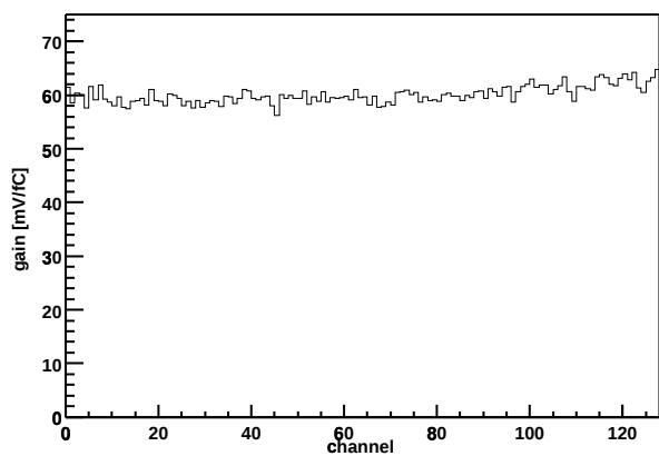
Chip Z36459A-W06-X10-Y10 Gain vs. channel
