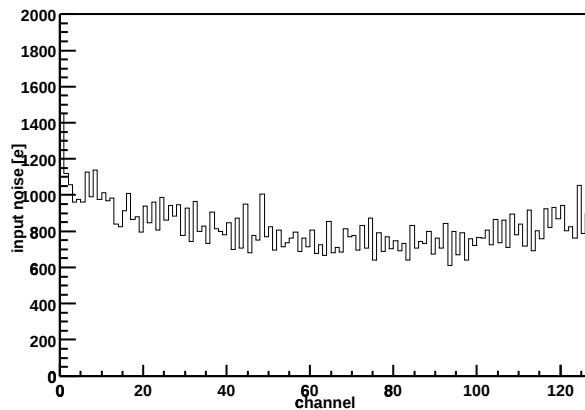
Chip Z36459A-W06-X10-Y10 Input noise vs. channel
