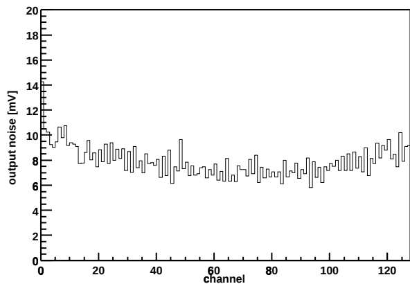
Chip Z36459A-W06-X10-Y10 Output noise vs. channel
