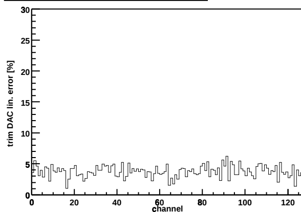
Chip Z36459A-W06-X10-Y13 trim DAC lin. error
