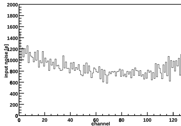
Chip Z36459A-W06-X10-Y13 Input noise vs. channel
