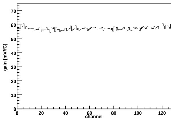
Chip Z36459A-W06-X10-Y13 Gain vs. channel
