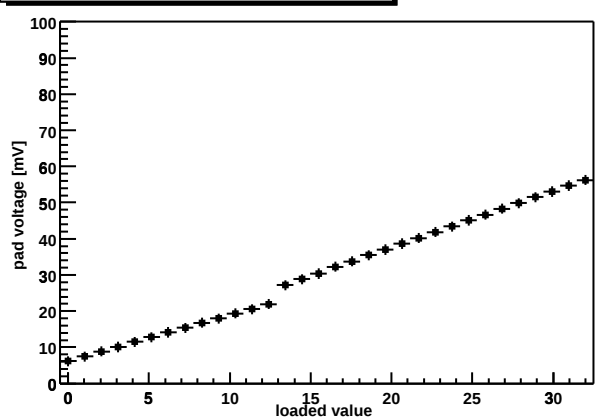
Chip Z36459A-W06-X10-Y13 shaper DAC
