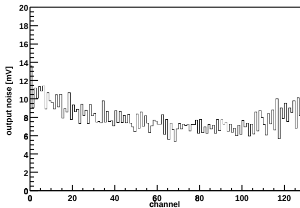
Chip Z36459A-W06-X10-Y13 Output noise vs. channel
