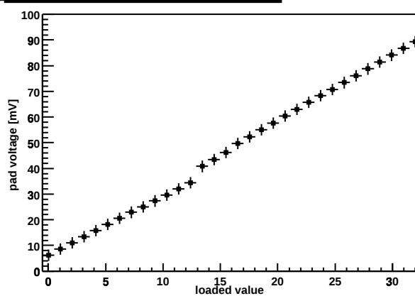
Chip Z36459A-W06-X10-Y13 preamp DAC
