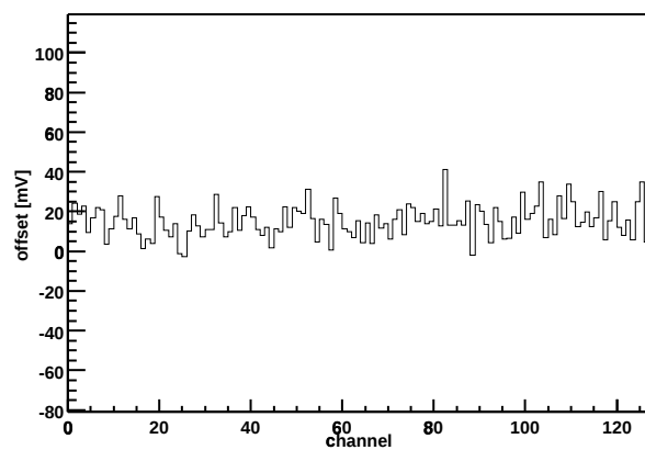
Chip Z36459A-W06-X10-Y13 Offset vs. channel
