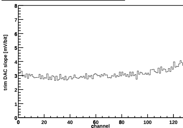
Chip Z36459A-W06-X10-Y13 Trim DAC slope vs. channel
