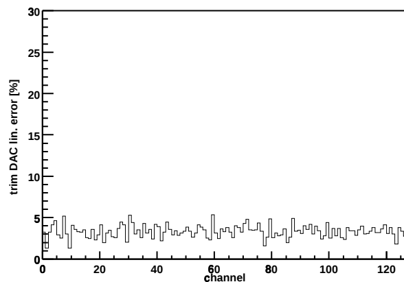
Chip Z36459A-W06-X10-Y15 trim DAC lin. error
