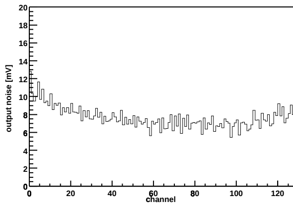
Chip Z36459A-W06-X10-Y15 Output noise vs. channel
