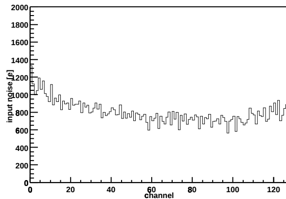
Chip Z36459A-W06-X10-Y15 Input noise vs. channel
