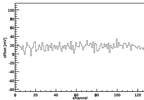
Chip Z36459A-W06-X10-Y15 Offset vs. channel
