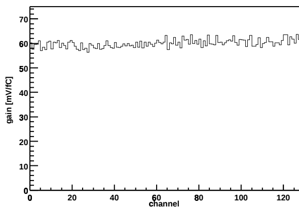
Chip Z36459A-W06-X10-Y15 Gain vs. channel
