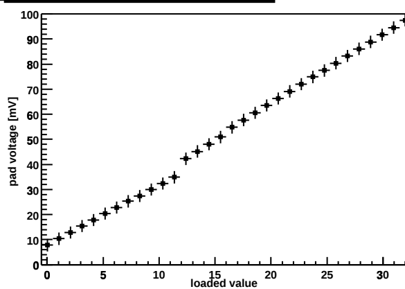
Chip Z36459A-W06-X10-Y15 preamp DAC
