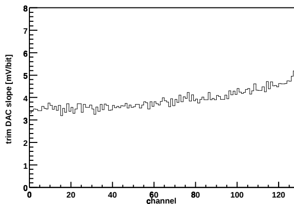
Chip Z36459A-W06-X10-Y15 Trim DAC slope vs. channel
