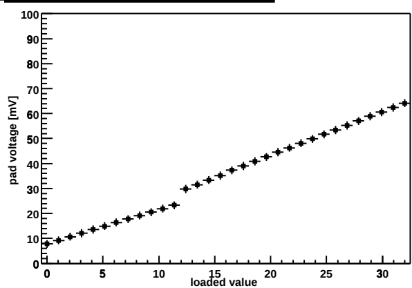
Chip Z36459A-W06-X10-Y15 shaper DAC
