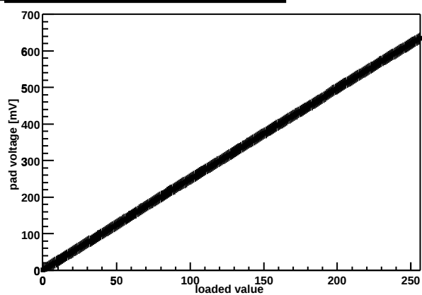
Chip Z36459A-W06-X10-Y15 threshold DAC
