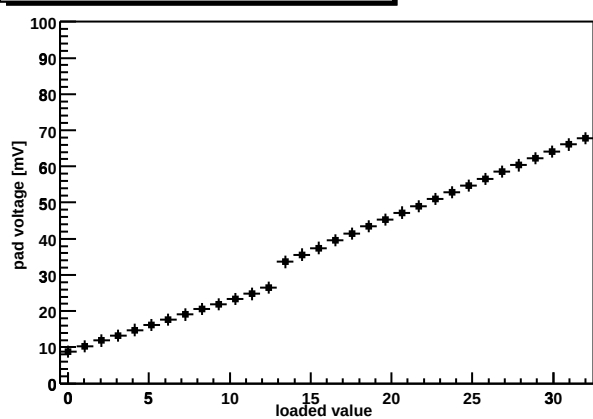
Chip Z36459A-W06-X10-Y16 shaper DAC
