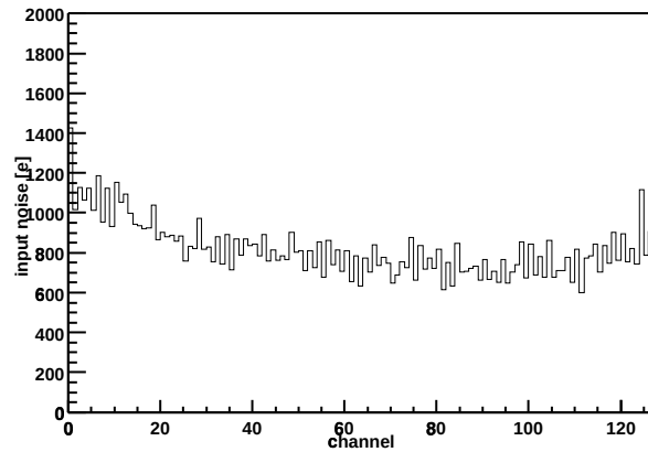
Chip Z36459A-W06-X10-Y16 Input noise vs. channel
