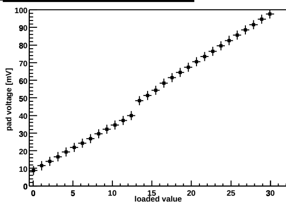
Chip Z36459A-W06-X10-Y16 preamp DAC
