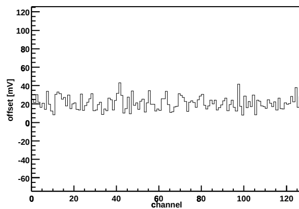
Chip Z36459A-W06-X10-Y16 Offset vs. channel
