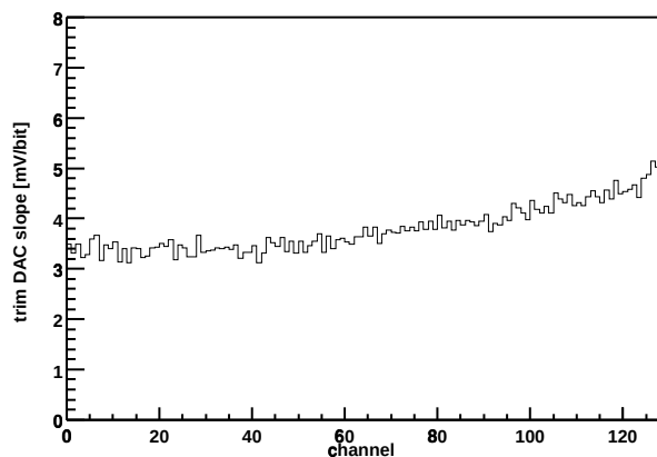
Chip Z36459A-W06-X10-Y16 Trim DAC slope vs. channel
