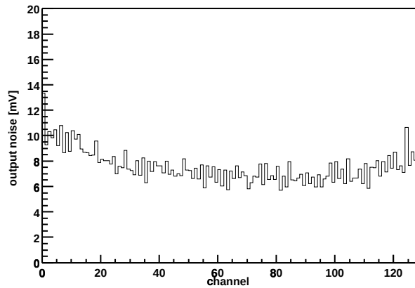
Chip Z36459A-W06-X10-Y16 Output noise vs. channel
