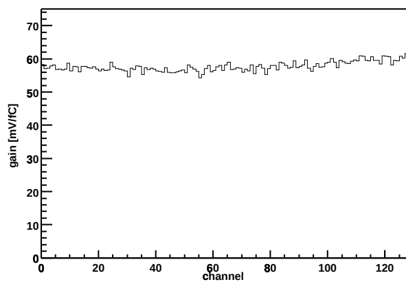
Chip Z36459A-W06-X10-Y16 Gain vs. channel
