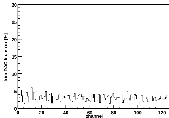
Chip Z36459A-W06-X10-Y16 trim DAC lin. error
