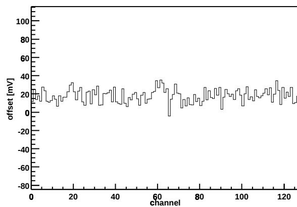
Chip Z36459A-W06-X10-Y17 Offset vs. channel
