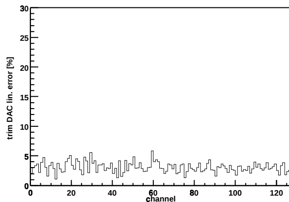
Chip Z36459A-W06-X10-Y17 trim DAC lin. error
