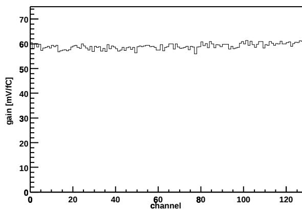
Chip Z36459A-W06-X10-Y17 Gain vs. channel
