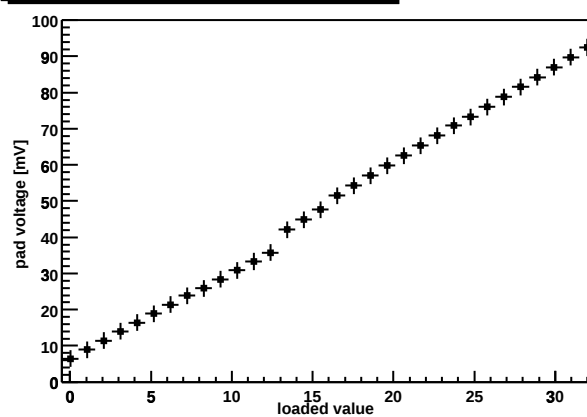
Chip Z36459A-W06-X10-Y17 preamp DAC
