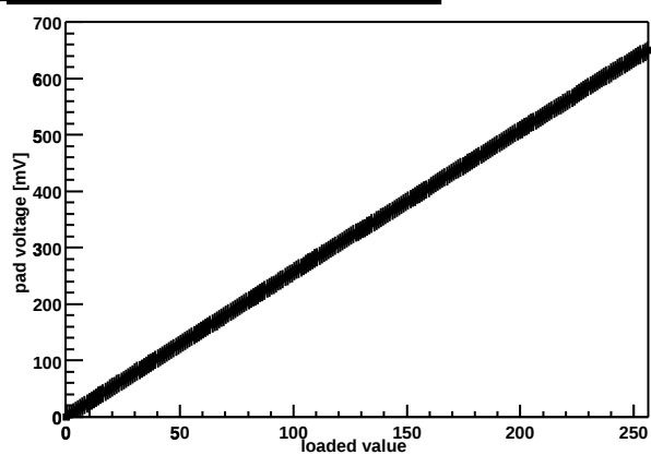
Chip Z36459A-W06-X10-Y17 threshold DAC
