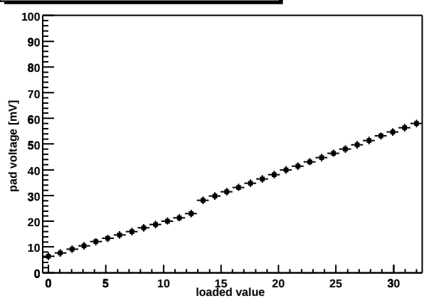
Chip Z36459A-W06-X10-Y17 shaper DAC
