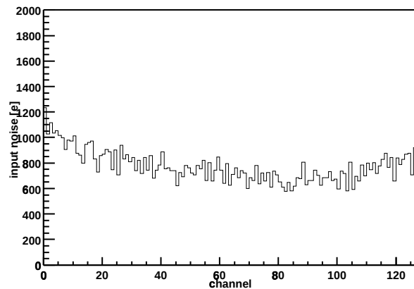
Chip Z36459A-W06-X10-Y17 Input noise vs. channel
