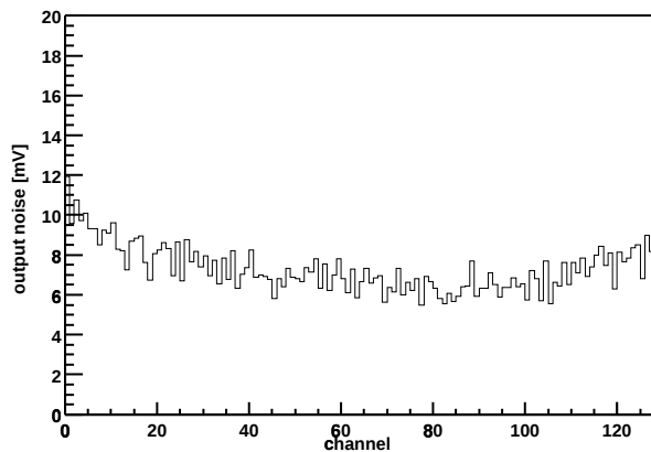
Chip Z36459A-W06-X10-Y17 Output noise vs. channel
