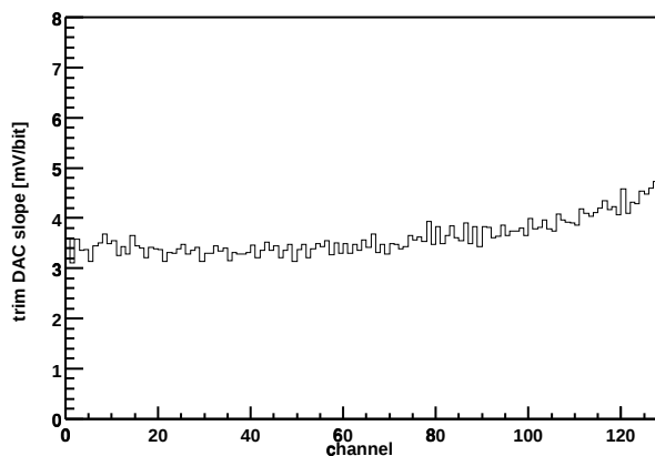
Chip Z36459A-W06-X10-Y17 Trim DAC slope vs. channel
