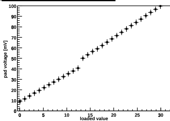
Chip Z36459A-W06-X11-Y04 preamp DAC
