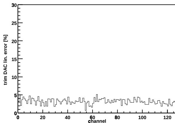
Chip Z36459A-W06-X11-Y04 trim DAC lin. error
