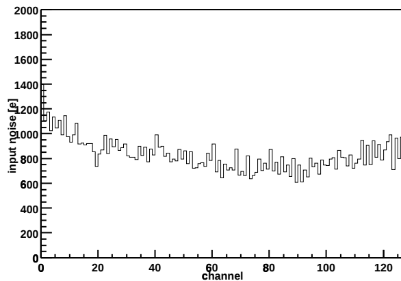
Chip Z36459A-W06-X11-Y04 Input noise vs. channel
