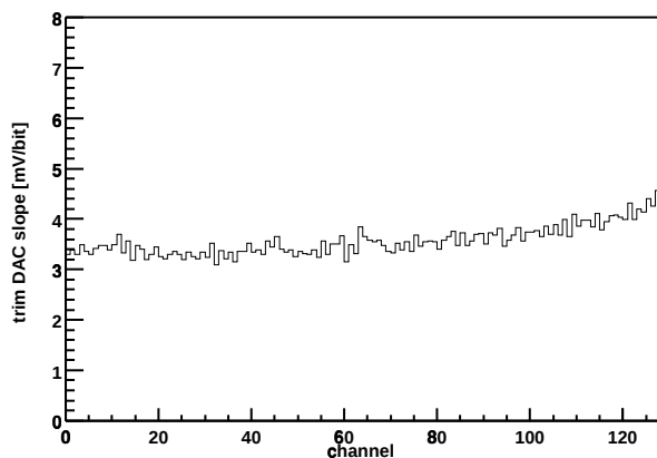
Chip Z36459A-W06-X11-Y04 Trim DAC slope vs. channel
