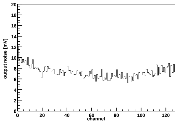
Chip Z36459A-W06-X11-Y04 Output noise vs. channel
