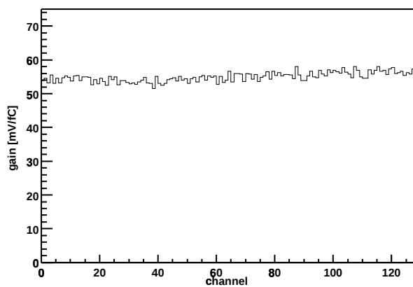
Chip Z36459A-W06-X11-Y04 Gain vs. channel
