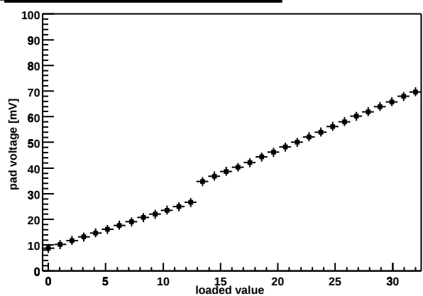
Chip Z36459A-W06-X11-Y04 shaper DAC
