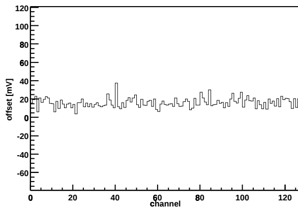
Chip Z36459A-W06-X11-Y04 Offset vs. channel
