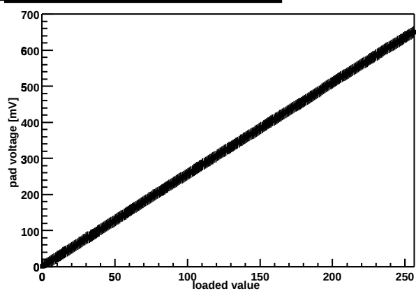
Chip Z36459A-W06-X11-Y04 threshold DAC
