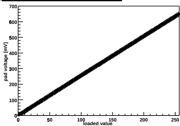
Chip Z36459A-W06-X11-Y05 threshold DAC
