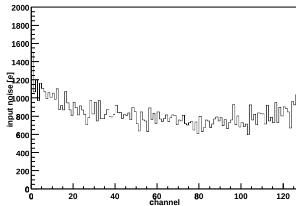
Chip Z36459A-W06-X11-Y05 Input noise vs. channel
