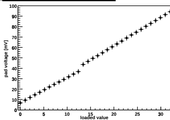
Chip Z36459A-W06-X11-Y05 preamp DAC
