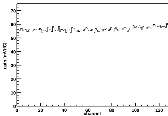
Chip Z36459A-W06-X11-Y05 Gain vs. channel
