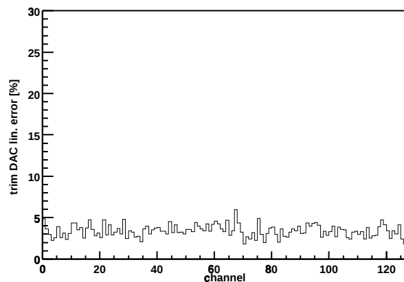
Chip Z36459A-W06-X11-Y05 trim DAC lin. error
