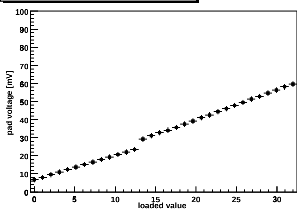
Chip Z36459A-W06-X11-Y05 shaper DAC
