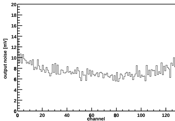
Chip Z36459A-W06-X11-Y05 Output noise vs. channel
