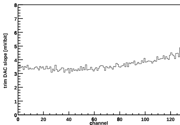
Chip Z36459A-W06-X11-Y05 Trim DAC slope vs. channel
