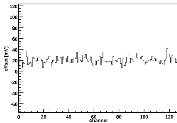
Chip Z36459A-W06-X11-Y05 Offset vs. channel
