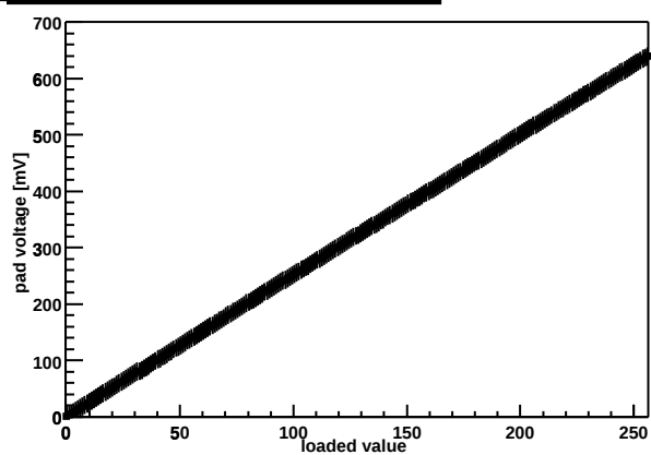
Chip Z36459A-W06-X11-Y11 threshold DAC
