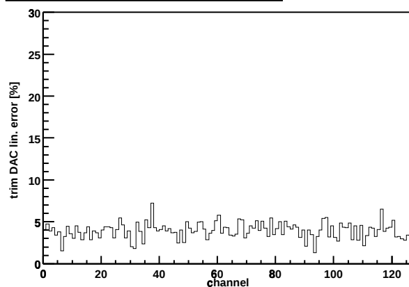
Chip Z36459A-W06-X11-Y11 trim DAC lin. error
