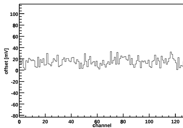
Chip Z36459A-W06-X11-Y11 Offset vs. channel
