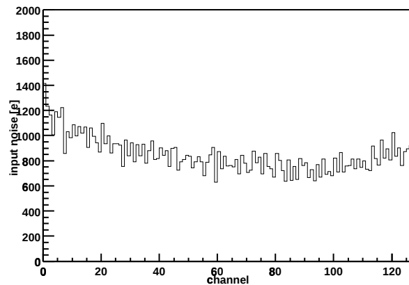
Chip Z36459A-W06-X11-Y11 Input noise vs. channel
