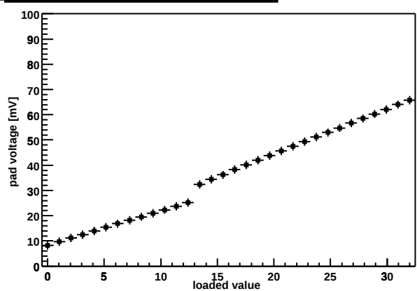
Chip Z36459A-W06-X11-Y11 shaper DAC
