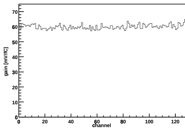
Chip Z36459A-W06-X11-Y11 Gain vs. channel
