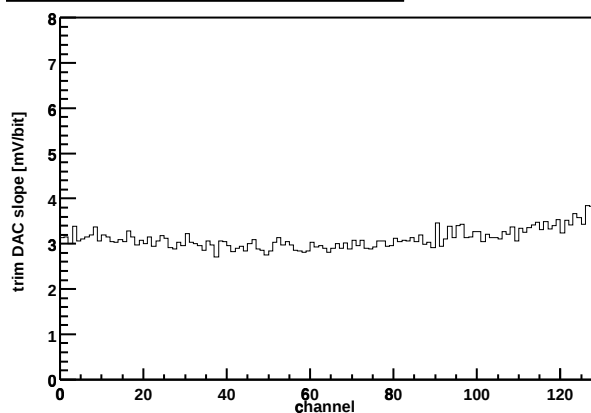
Chip Z36459A-W06-X11-Y11 Trim DAC slope vs. channel
