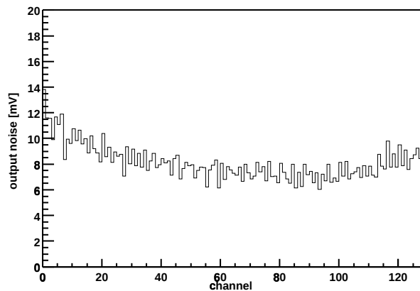
Chip Z36459A-W06-X11-Y11 Output noise vs. channel
