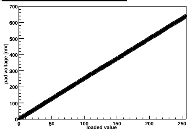
Chip Z36459A-W06-X11-Y12 threshold DAC
