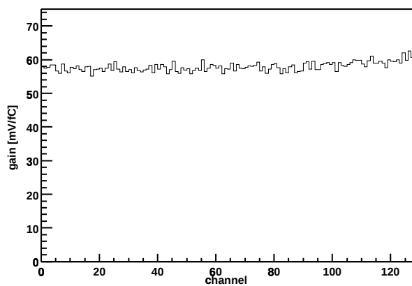
Chip Z36459A-W06-X11-Y12 Gain vs. channel
