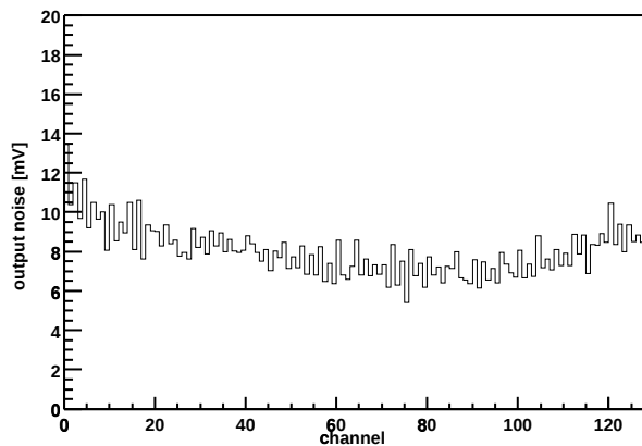
Chip Z36459A-W06-X11-Y12 Output noise vs. channel
