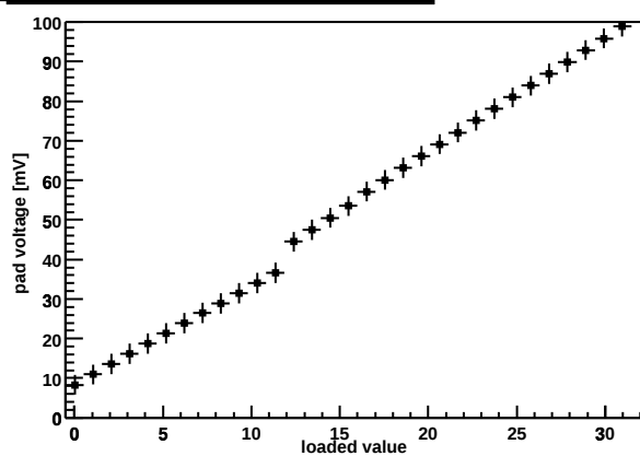
Chip Z36459A-W06-X11-Y12 preamp DAC
