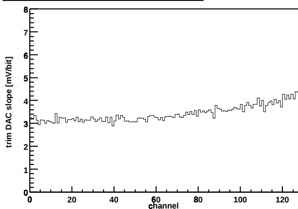
Chip Z36459A-W06-X11-Y12 Trim DAC slope vs. channel
