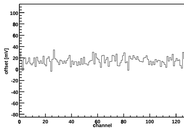
Chip Z36459A-W06-X11-Y12 Offset vs. channel
