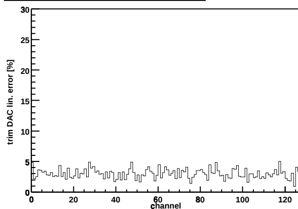
Chip Z36459A-W06-X11-Y12 trim DAC lin. error
