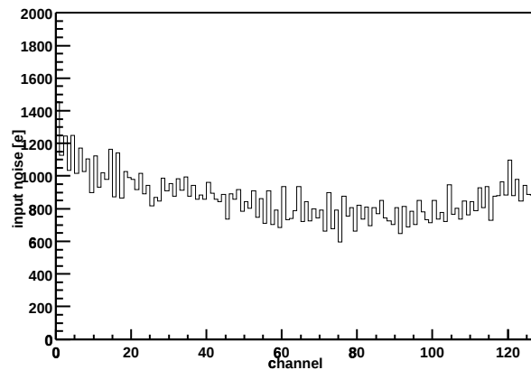
Chip Z36459A-W06-X11-Y12 Input noise vs. channel
