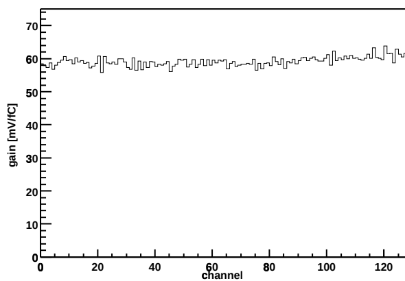
Chip Z36459A-W06-X11-Y13 Gain vs. channel
