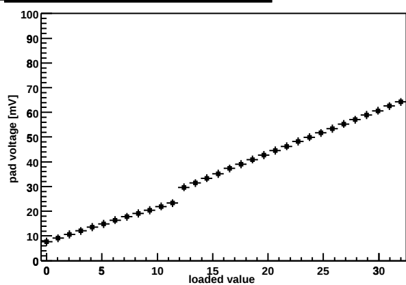
Chip Z36459A-W06-X11-Y13 shaper DAC
