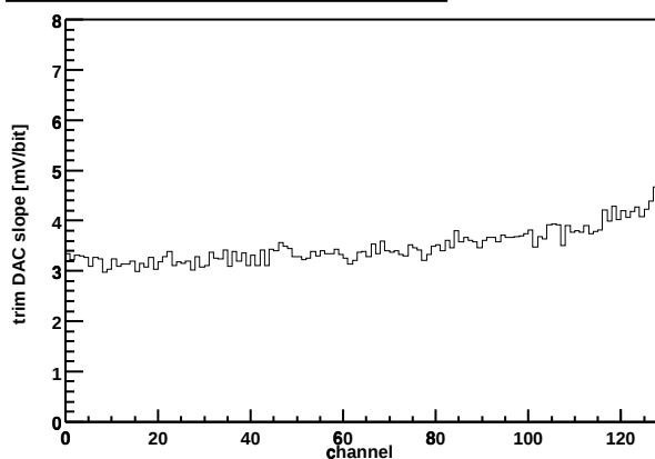
Chip Z36459A-W06-X11-Y13 Trim DAC slope vs. channel
