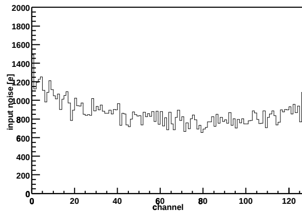
Chip Z36459A-W06-X11-Y13 Input noise vs. channel
