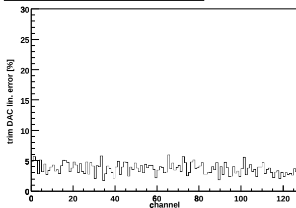
Chip Z36459A-W06-X11-Y13 trim DAC lin. error
