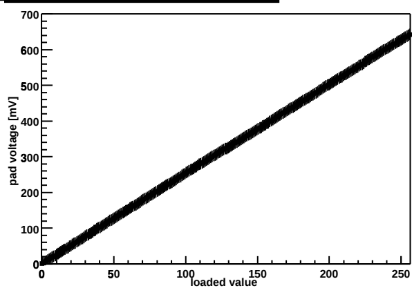
Chip Z36459A-W06-X11-Y13 threshold DAC
