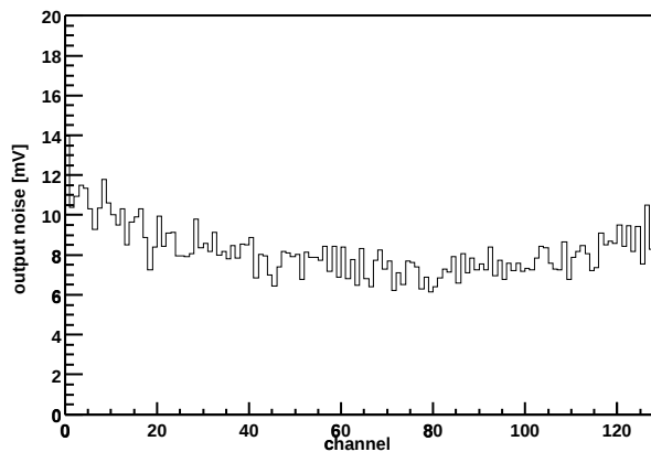
Chip Z36459A-W06-X11-Y13 Output noise vs. channel
