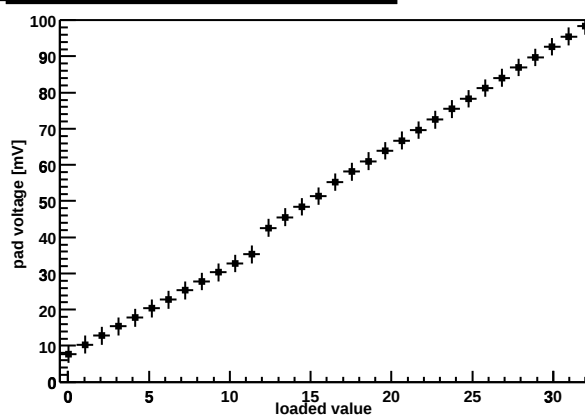
Chip Z36459A-W06-X11-Y13 preamp DAC
