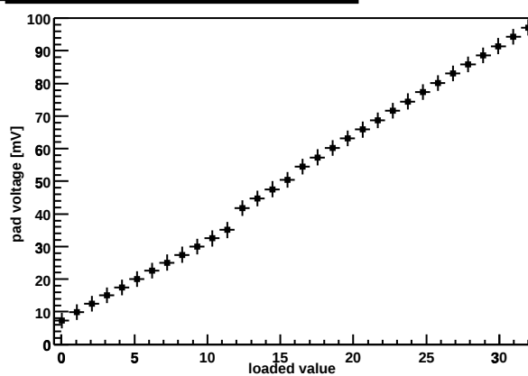
Chip Z36459A-W06-X11-Y15 preamp DAC
