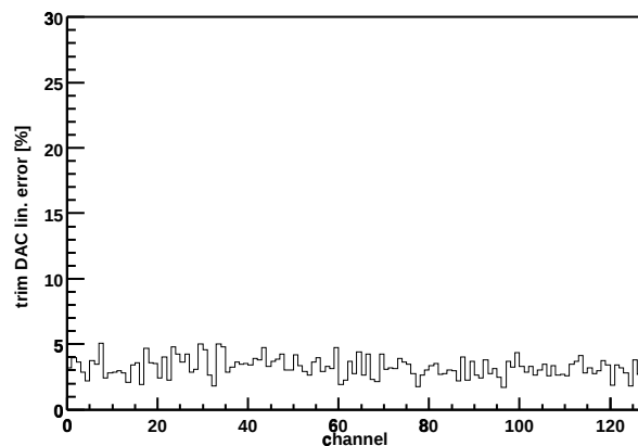
Chip Z36459A-W06-X11-Y15 trim DAC lin. error
