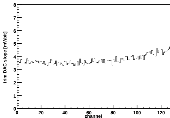
Chip Z36459A-W06-X11-Y15 Trim DAC slope vs. channel
