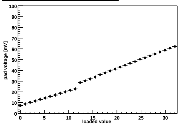
Chip Z36459A-W06-X11-Y15 shaper DAC
