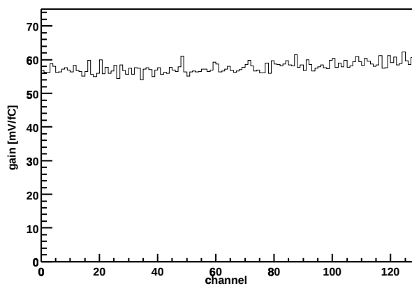
Chip Z36459A-W06-X11-Y15 Gain vs. channel
