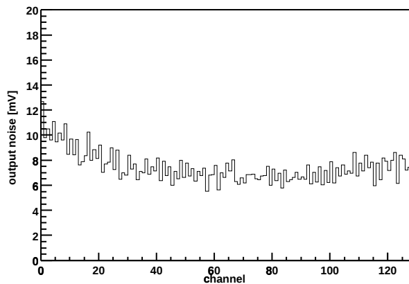
Chip Z36459A-W06-X11-Y15 Output noise vs. channel
