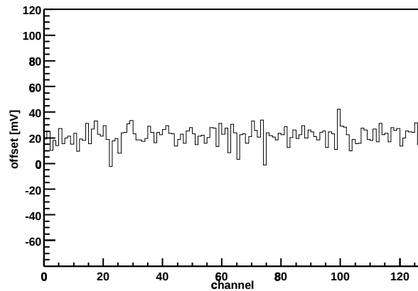
Chip Z36459A-W06-X11-Y15 Offset vs. channel
