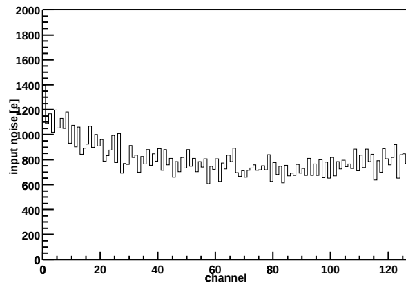
Chip Z36459A-W06-X11-Y15 Input noise vs. channel
