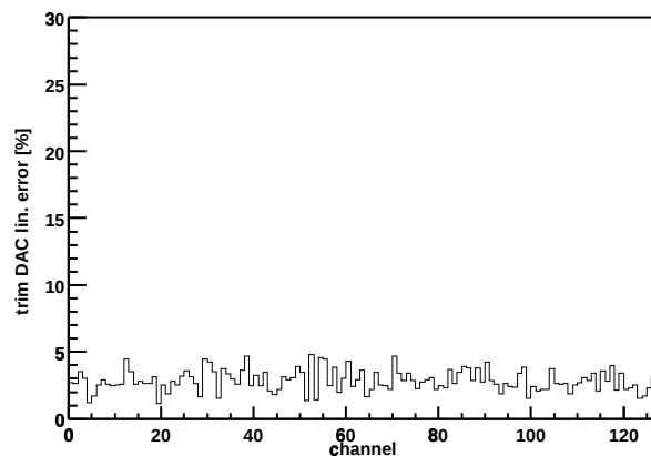
Chip Z36459A-W06-X11-Y16 trim DAC lin. error
