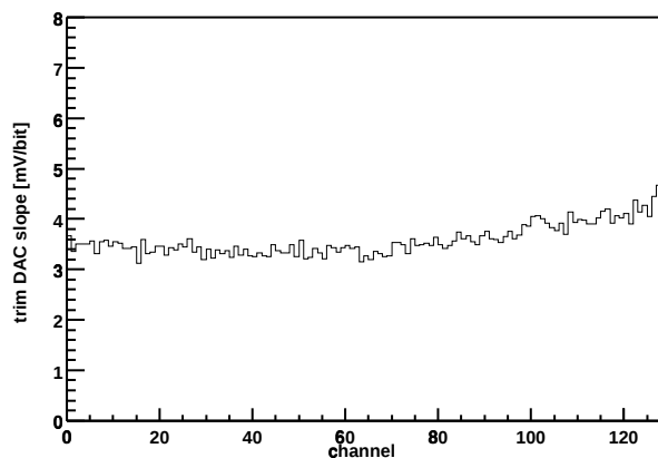
Chip Z36459A-W06-X11-Y16 Trim DAC slope vs. channel
