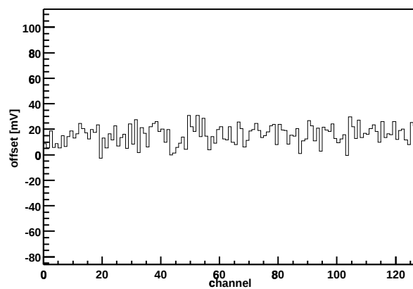
Chip Z36459A-W06-X11-Y16 Offset vs. channel
