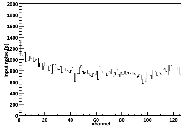
Chip Z36459A-W06-X11-Y16 Input noise vs. channel
