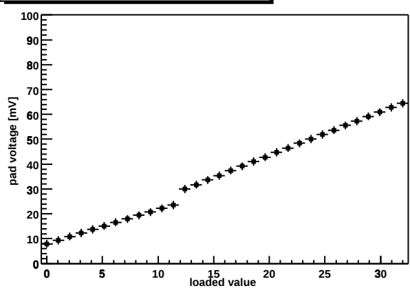
Chip Z36459A-W06-X11-Y16 shaper DAC
