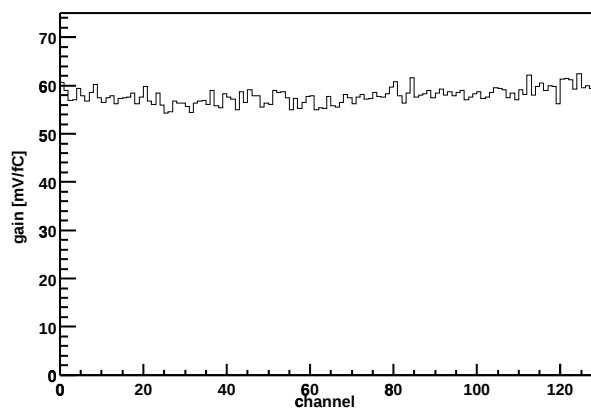
Chip Z36459A-W06-X11-Y16 Gain vs. channel
