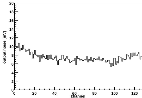
Chip Z36459A-W06-X11-Y16 Output noise vs. channel
