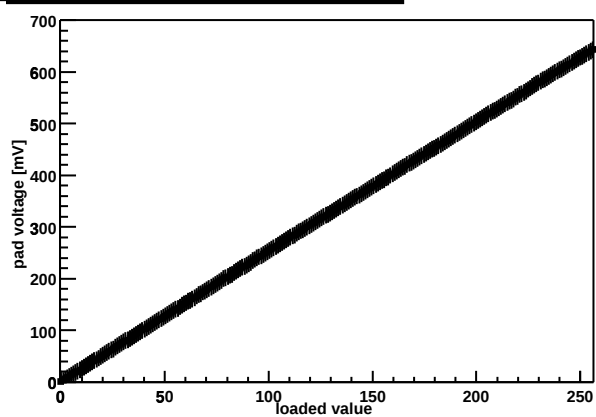
Chip Z36459A-W06-X11-Y16 threshold DAC
