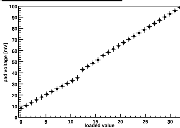
Chip Z36459A-W06-X11-Y16 preamp DAC
