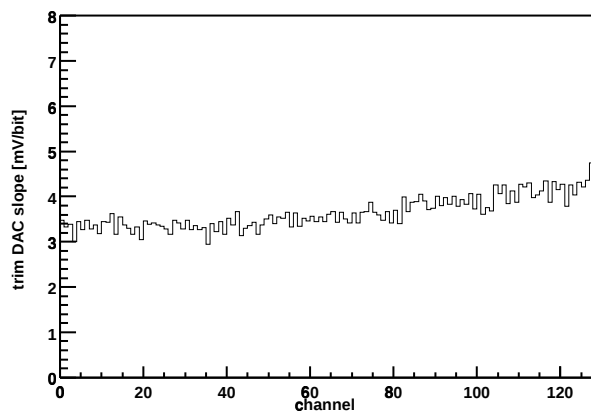
Chip Z36459A-W06-X11-Y17 Trim DAC slope vs. channel
