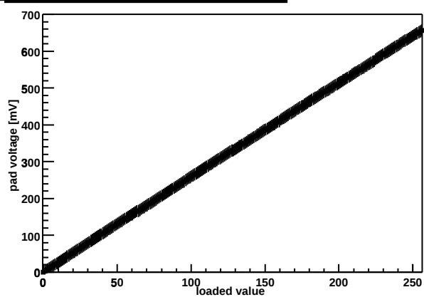
Chip Z36459A-W06-X11-Y17 threshold DAC
