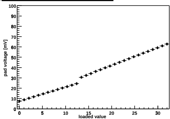
Chip Z36459A-W06-X11-Y17 shaper DAC
