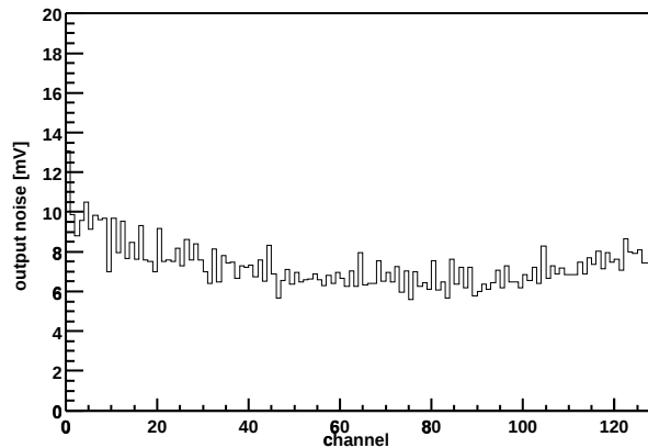
Chip Z36459A-W06-X11-Y17 Output noise vs. channel
