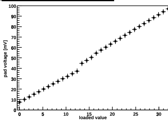
Chip Z36459A-W06-X11-Y17 preamp DAC
