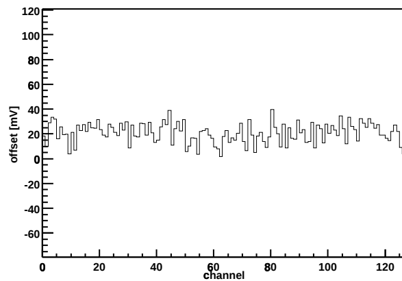
Chip Z36459A-W06-X11-Y17 Offset vs. channel
