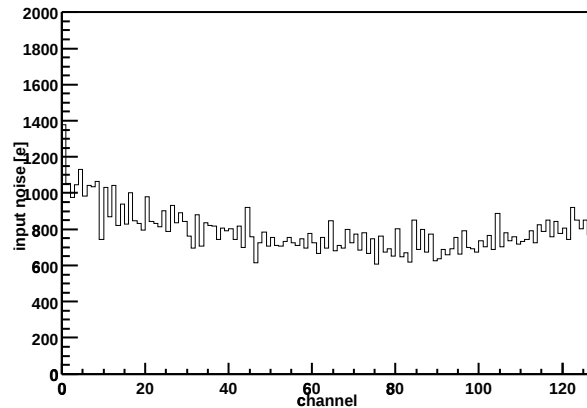
Chip Z36459A-W06-X11-Y17 Input noise vs. channel
