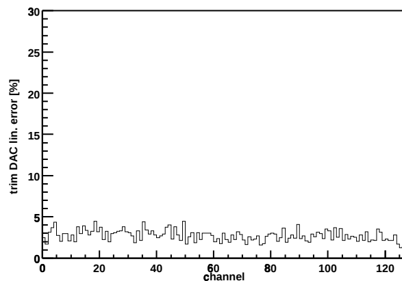
Chip Z36459A-W06-X11-Y17 trim DAC lin. error
