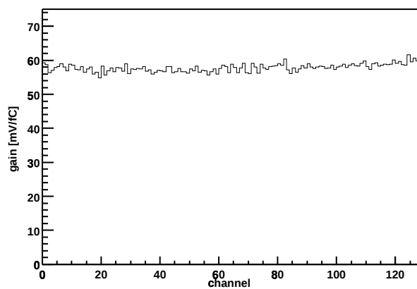
Chip Z36459A-W06-X11-Y17 Gain vs. channel
