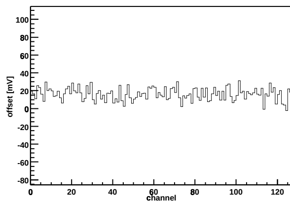
Chip Z36459A-W06-X12-Y09 Offset vs. channel
