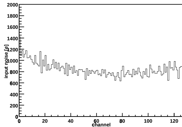
Chip Z36459A-W06-X12-Y09 Input noise vs. channel
