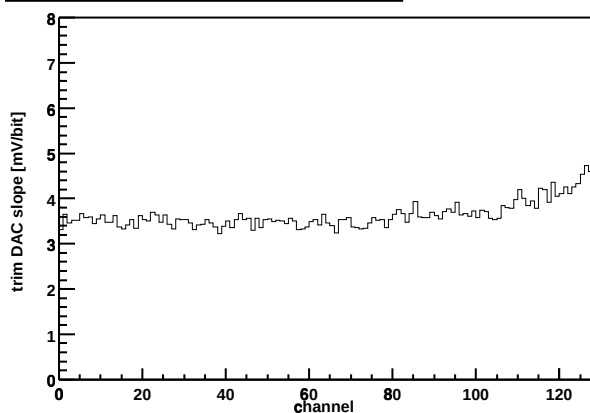
Chip Z36459A-W06-X12-Y09 Trim DAC slope vs. channel
