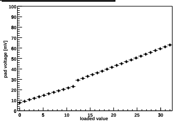
Chip Z36459A-W06-X12-Y09 shaper DAC
