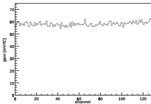
Chip Z36459A-W06-X12-Y09 Gain vs. channel
