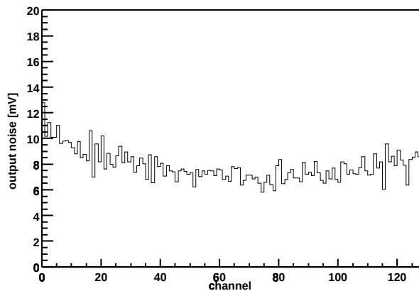
Chip Z36459A-W06-X12-Y09 Output noise vs. channel
