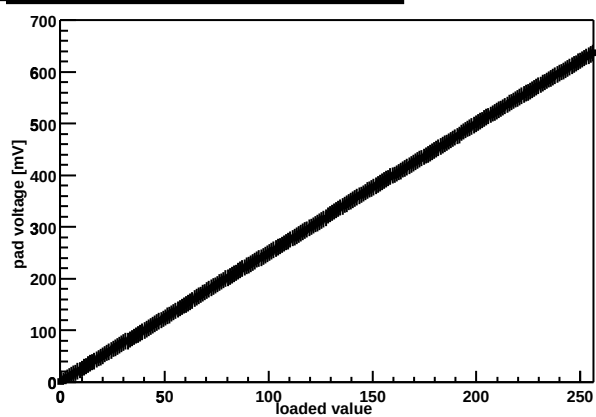
Chip Z36459A-W06-X12-Y09 threshold DAC
