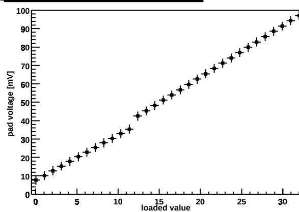
Chip Z36459A-W06-X12-Y09 preamp DAC
