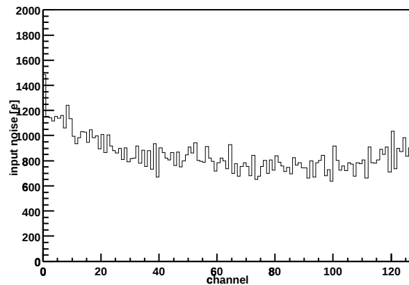
Chip Z36459A-W06-X12-Y12 Input noise vs. channel
