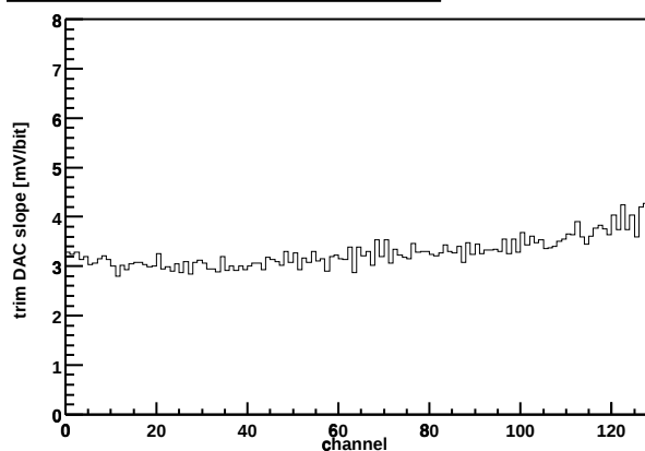
Chip Z36459A-W06-X12-Y12 Trim DAC slope vs. channel
