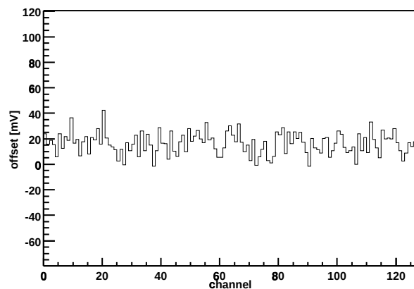
Chip Z36459A-W06-X12-Y12 Offset vs. channel
