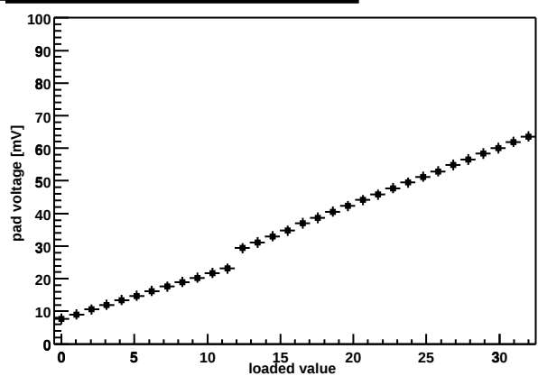
Chip Z36459A-W06-X12-Y12 shaper DAC
