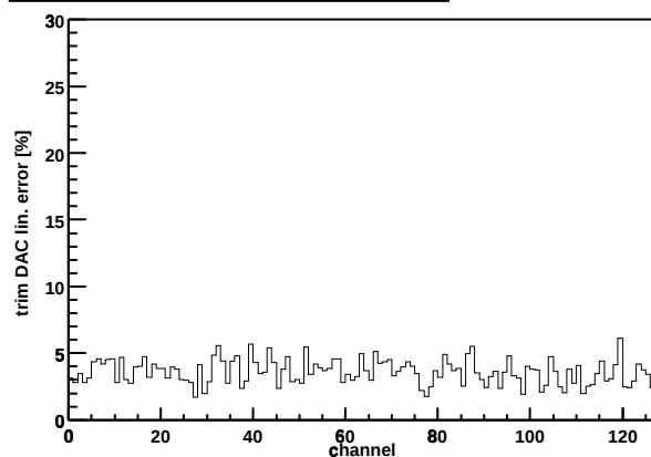
Chip Z36459A-W06-X12-Y12 trim DAC lin. error
