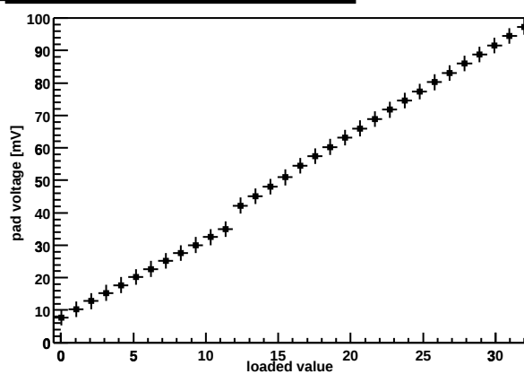
Chip Z36459A-W06-X12-Y12 preamp DAC
