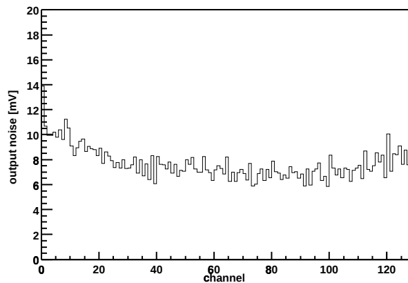
Chip Z36459A-W06-X12-Y12 Output noise vs. channel
