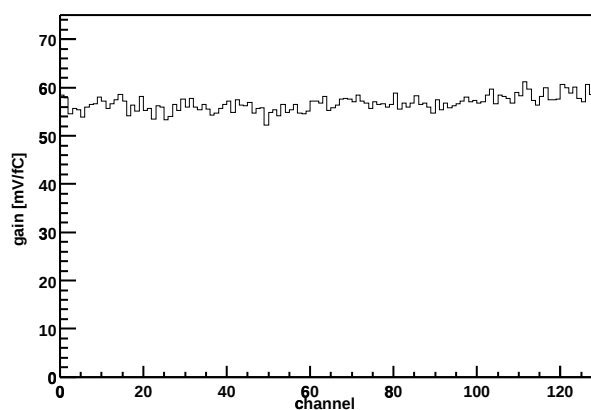
Chip Z36459A-W06-X12-Y12 Gain vs. channel
