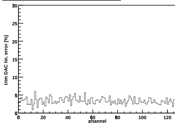
Chip Z36459A-W06-X12-Y13 trim DAC lin. error
