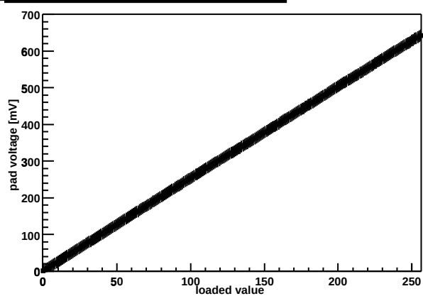
Chip Z36459A-W06-X12-Y13 threshold DAC
