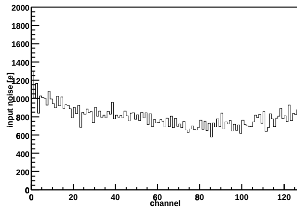
Chip Z36459A-W06-X12-Y13 Input noise vs. channel
