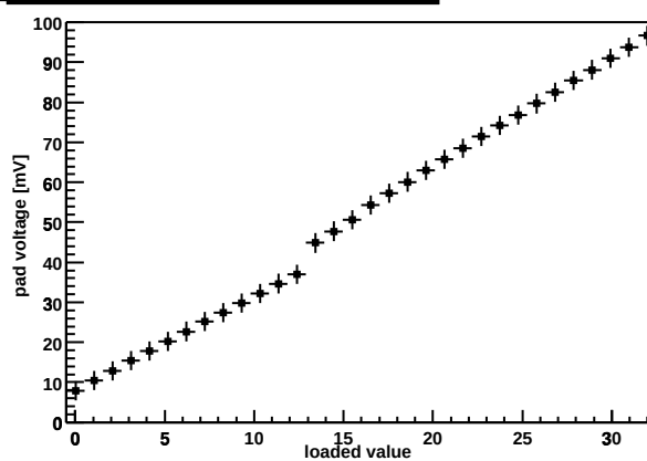
Chip Z36459A-W06-X12-Y13 preamp DAC
