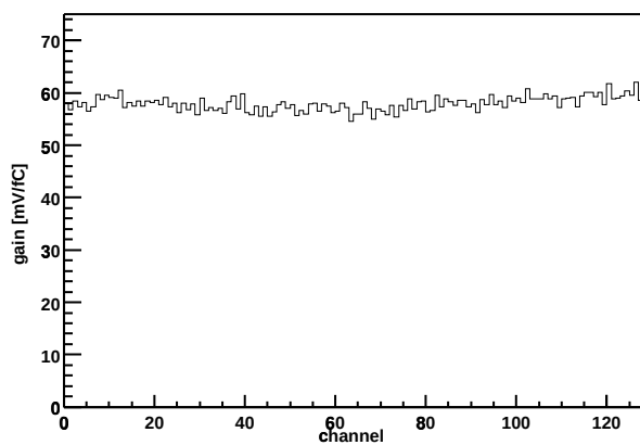
Chip Z36459A-W06-X12-Y13 Gain vs. channel
