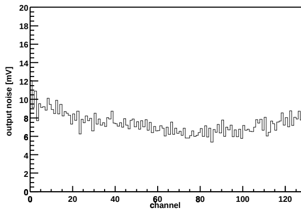
Chip Z36459A-W06-X12-Y13 Output noise vs. channel
