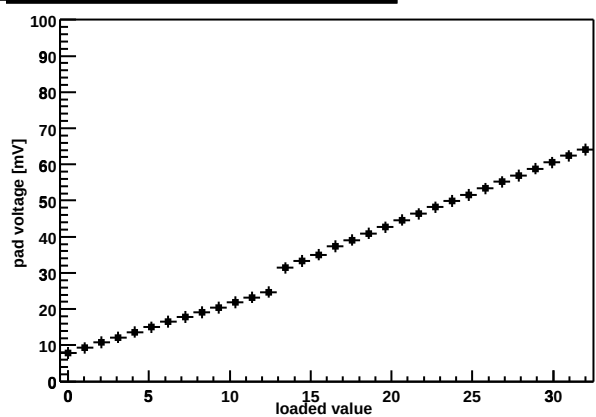
Chip Z36459A-W06-X12-Y13 shaper DAC
