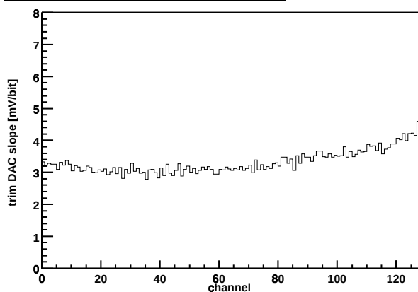
Chip Z36459A-W06-X12-Y13 Trim DAC slope vs. channel
