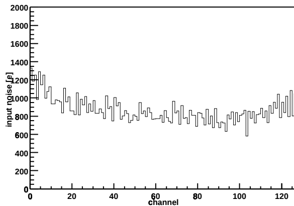
Chip Z36459A-W06-X13-Y08 Input noise vs. channel
