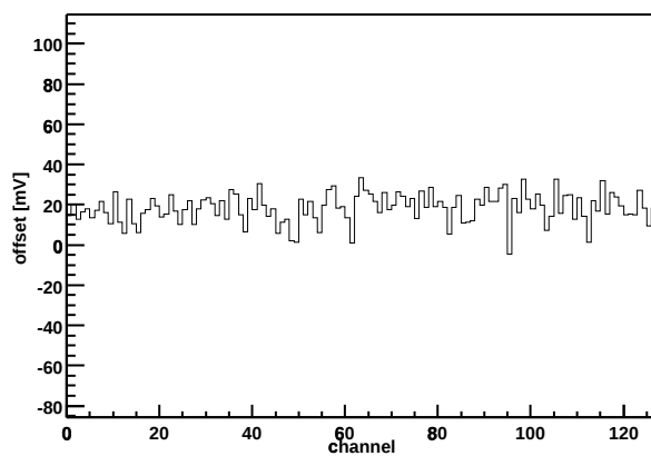
Chip Z36459A-W06-X13-Y08 Offset vs. channel
