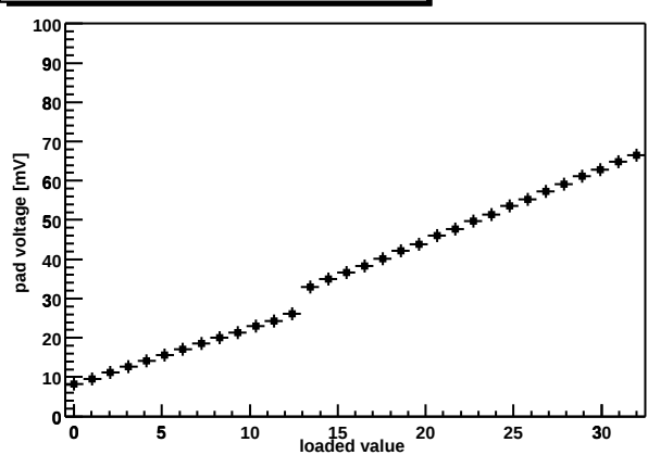
Chip Z36459A-W06-X13-Y08 shaper DAC
