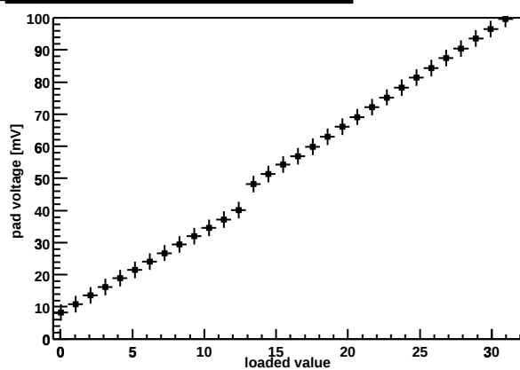
Chip Z36459A-W06-X13-Y08 preamp DAC
