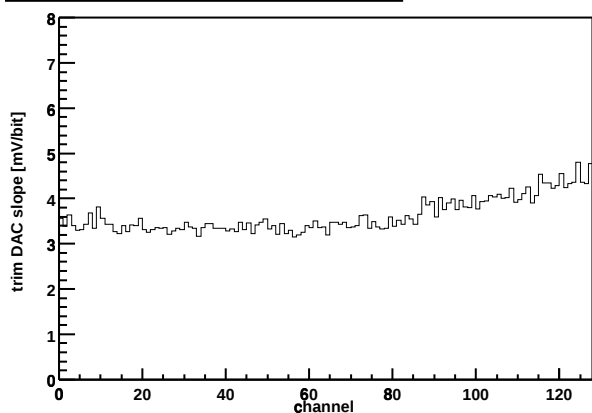
Chip Z36459A-W06-X13-Y08 Trim DAC slope vs. channel
