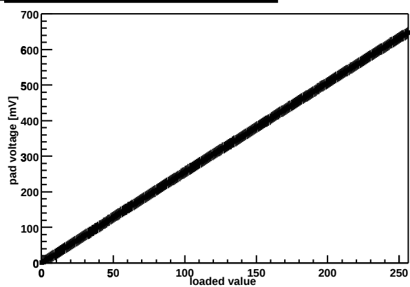
Chip Z36459A-W06-X13-Y08 threshold DAC
