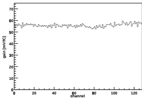
Chip Z36459A-W06-X13-Y08 Gain vs. channel
