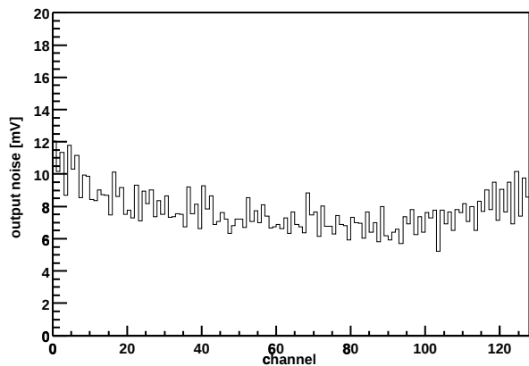
Chip Z36459A-W06-X13-Y08 Output noise vs. channel
