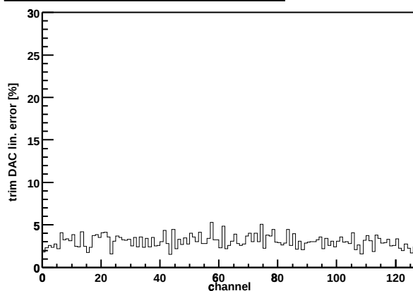
Chip Z36459A-W06-X13-Y08 trim DAC lin. error
