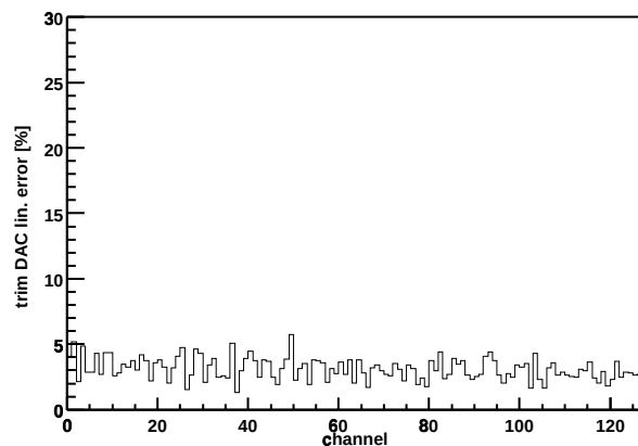
Chip Z36459A-W06-X13-Y10 trim DAC lin. error
