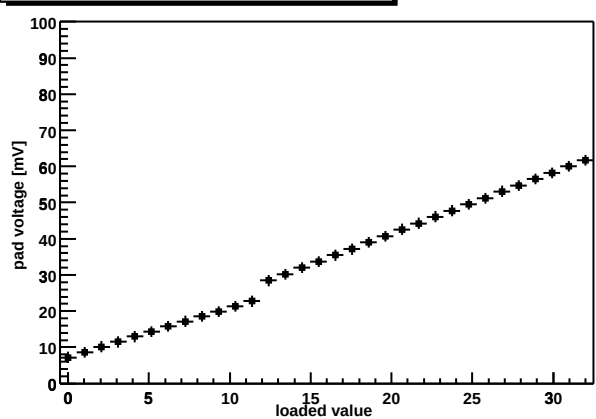
Chip Z36459A-W06-X13-Y10 shaper DAC
