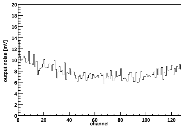
Chip Z36459A-W06-X13-Y10 Output noise vs. channel
