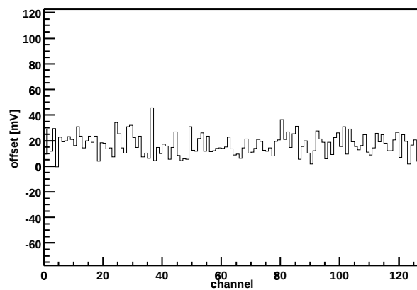
Chip Z36459A-W06-X13-Y10 Offset vs. channel
