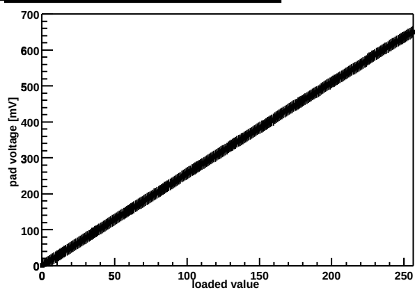
Chip Z36459A-W06-X13-Y10 threshold DAC
