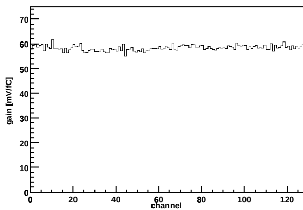
Chip Z36459A-W06-X13-Y10 Gain vs. channel
