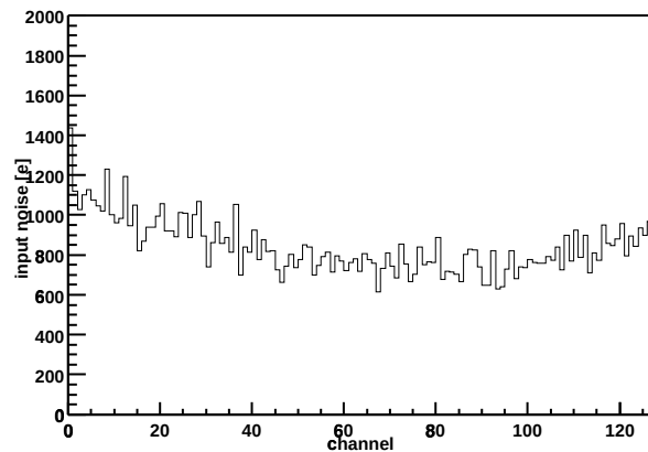
Chip Z36459A-W06-X13-Y10 Input noise vs. channel
