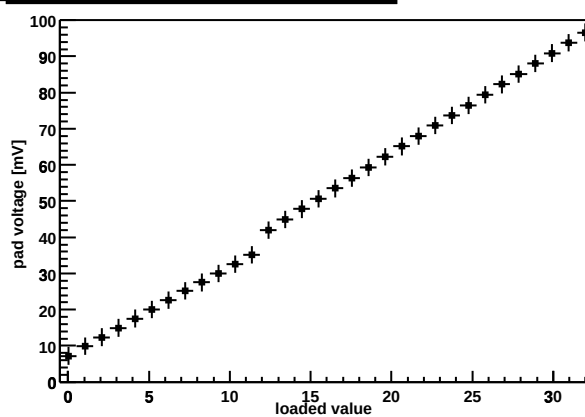
Chip Z36459A-W06-X13-Y10 preamp DAC
