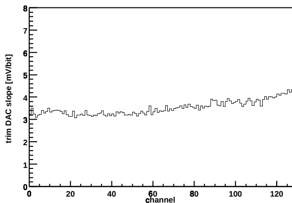
Chip Z36459A-W06-X13-Y10 Trim DAC slope vs. channel
